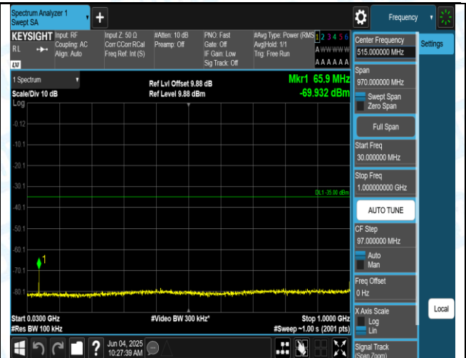
Band7-15MHz-QPSK-21100-1RB#0-30-1000-PASS
