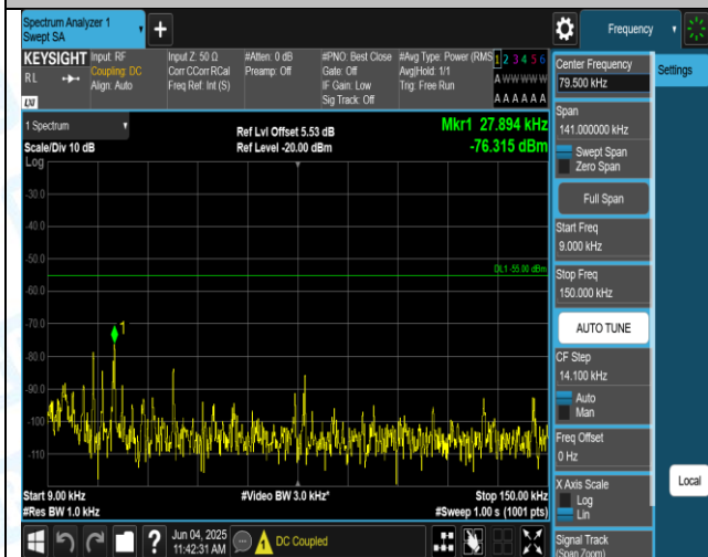
Band7-15MHz-QPSK-21375-1RB#0-0.009-0.15-PASS
