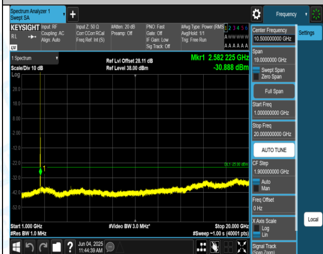
Band7-15MHz-16QAM-21375-1RB#0-1000-20000-PASS
