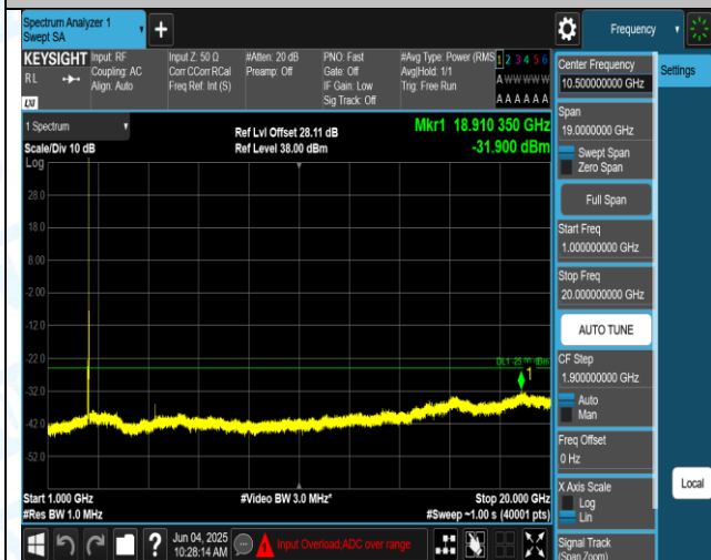
Band7-15MHz-QPSK-21100-1RB#0-1000-20000-PASS
