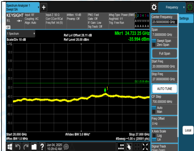
Band7-15MHz-16QAM-21100-1RB#0-20000~27000-PASS
