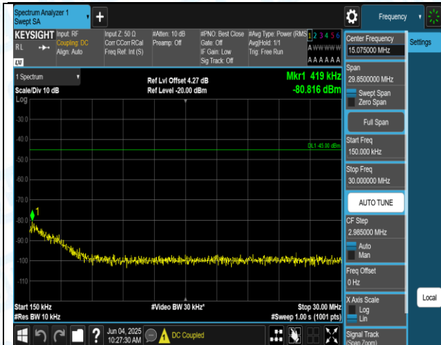
Band7-15MHz-QPSK-21100-1RB#0-0.15-30-PASS
