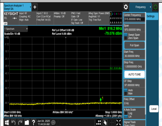
Band7-15MHz-16QAM-21375-1RB#0-30-1000-PASS
