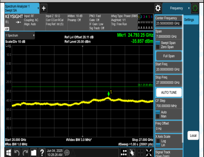
Band7-15MHz-QPSK-21100-1RB#0-20000-27000-PASS
