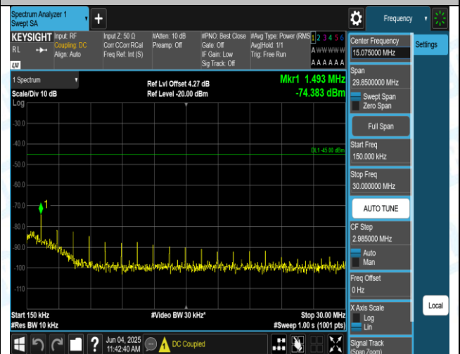
Band7-15MHz-QPSK-21375-1RB#0-0.15-30-PASS
