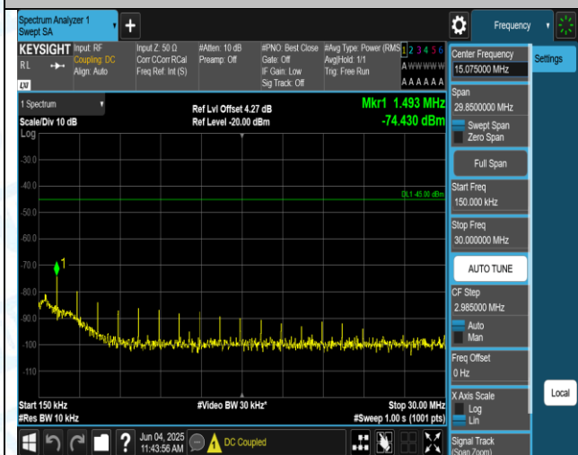
Band7-15MHz-16QAM-21375-1RB#0-0.15-30-PASS
