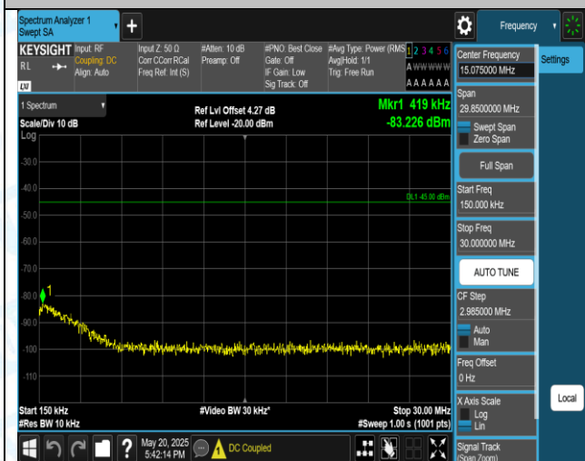
Band7-5MHz-16QAM-21425-1RB#0-0.15~30-PASS
