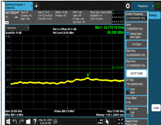
Band7-5MHz-16QAM-21100-1RB#0-20000~27000-PASS
