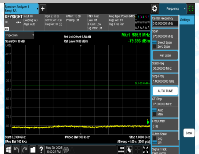
Band7-5MHz-16QAM-21425-1RB#0-30~1000-PASS
