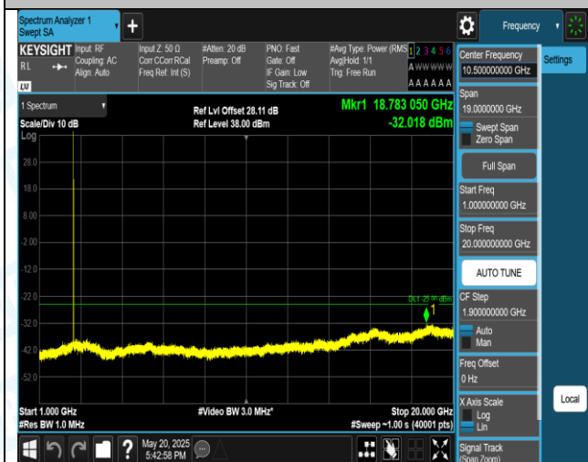
Band7-5MHz-16QAM-21425-1RB#0-1000~20000-PASS
