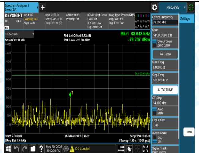
Band7-5MHz-16QAM-21425-1RB#0-0.009~0.15-PASS
