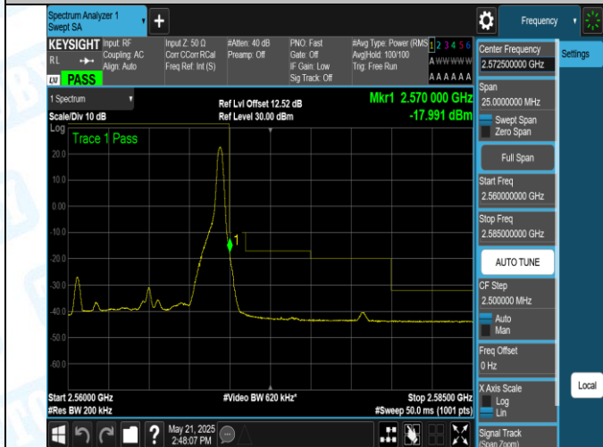
Band7-10MHz-16QAM-21400-1RB#49-PASS
