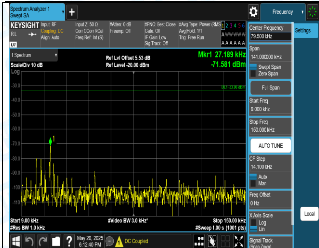
Band5-5MHz-QPSK-20425-1RB#0-0.009~0.15-PASS
