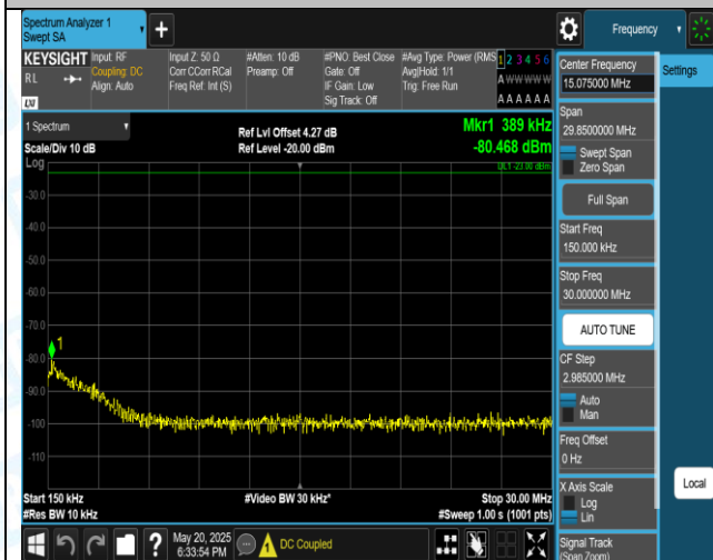
Band5-10MHz-16QAM-20450-1RB#0-0.15~30-PASS
