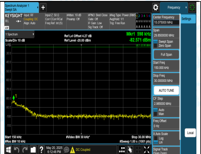
Band5-5MHz-QPSK-20425-1RB#0-0.15~30-PASS
