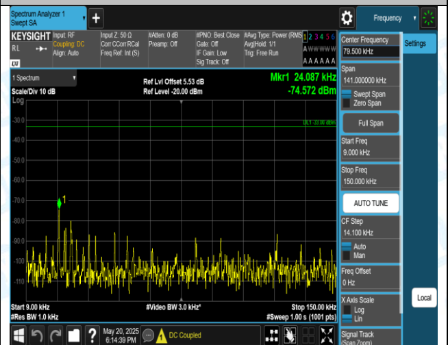
Band5-5MHz-QPSK-20525-1RB#0-0.009~0.15-PASS
