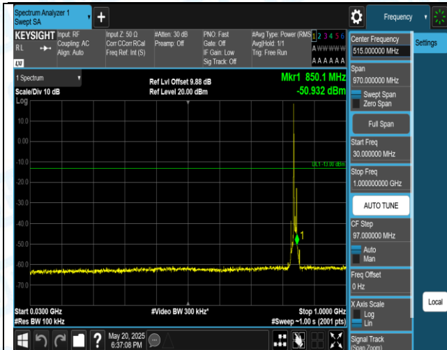
Band5-10MHz-QPSK-20600-1RB#0-30~1000-PASS
