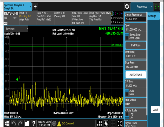
Band5-10MHz-16QAM-20450-1RB#0-0.009~0.15-PASS
