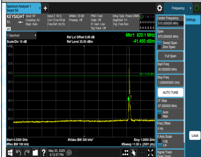
Band5-5MHz-QPSK-20425-1RB#0-30~1000-PASS
