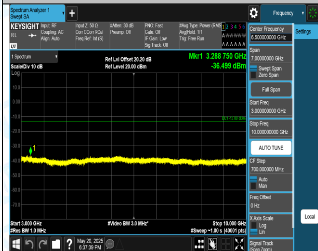
Band5-10MHz-QPSK-20600-1RB#0-3000~10000-PASS
