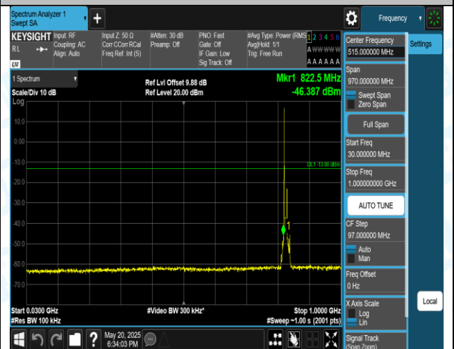
Band5-10MHz-16QAM-20450-1RB#0-30~1000-PASS
