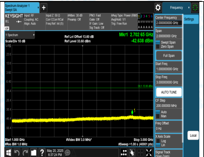
Band5-10MHz-QPSK-20600-1RB#0-1000~3000-PASS
