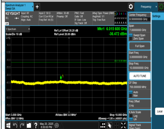
Band5-1.4MHz-QPSK-20643-1RB#0-3000-10000-PASS
