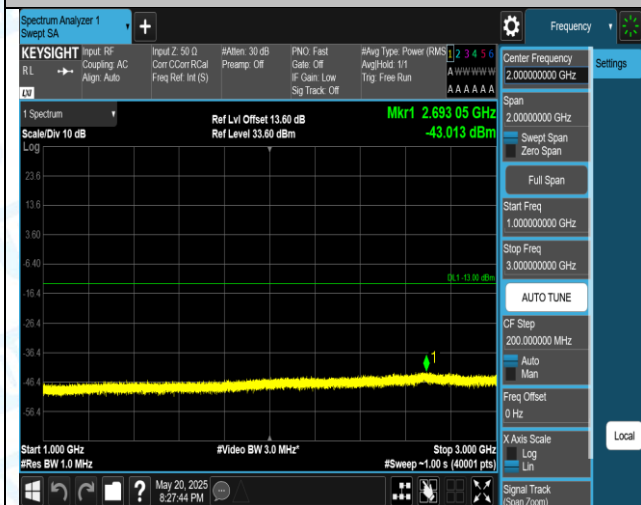
Band5-1.4MHz-QPSK-20525-1RB#0-1000-3000-PASS
