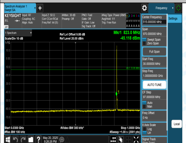
Band5-1.4MHz-16QAM-20407-1RB#0-30-1000-PASS
