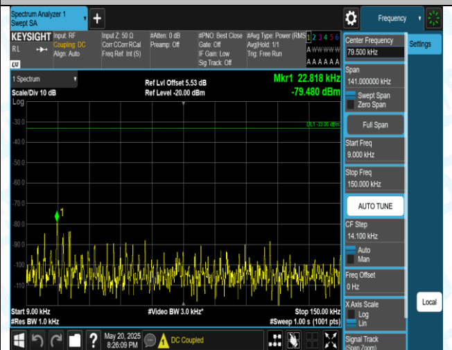
Band5-1.4MHz-16QAM-20407-1RB#0-0.009-0.15-PASS
