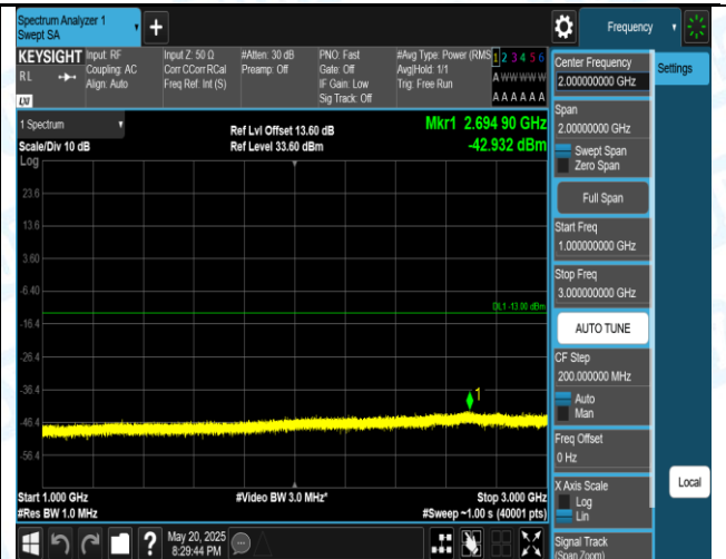
Band5-1.4MHz-QPSK-20643-1RB#0-1000-3000-PASS
