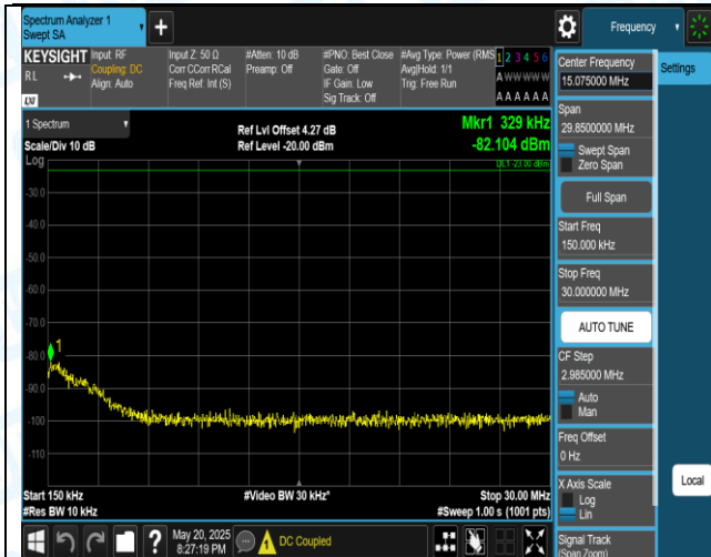
Band5-1.4MHz-QPSK-20525-1RB#0-0.15-30-PASS
