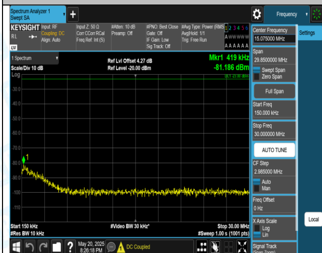
Band5-1.4MHz-16QAM-20407-1RB#0-0.15-30-PASS
