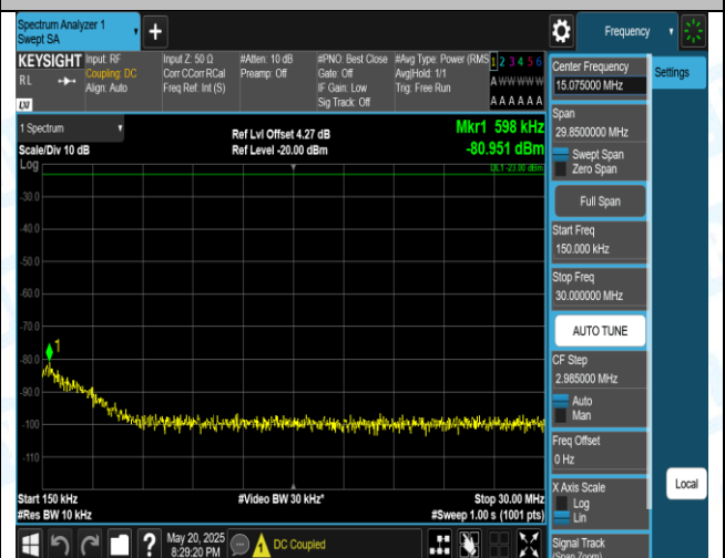
Band5-1.4MHz-QPSK-20643-1RB#0-0.15-30-PASS
