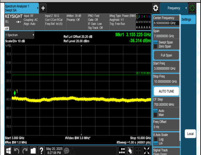
Band5-1.4MHz-QPSK-20525-1RB#0-3000-10000-PASS
