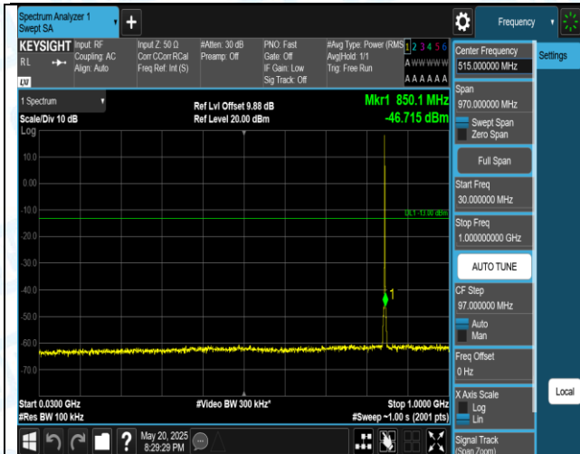
Band5-1.4MHz-QPSK-20643-1RB#0-30-1000-PASS
