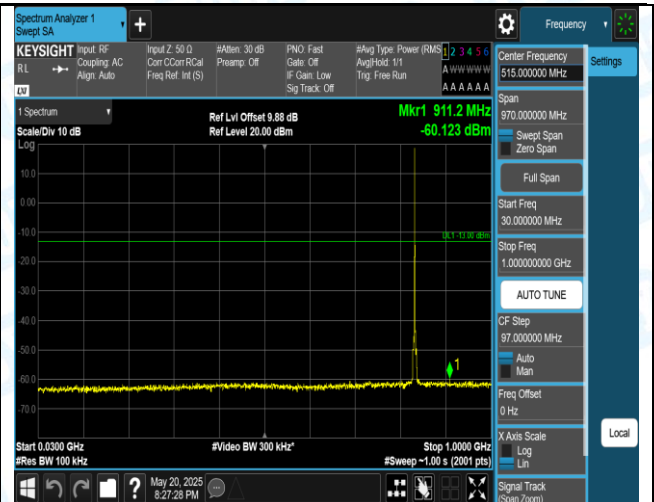
Band5-1.4MHz-QPSK-20525-1RB#0-30-1000-PASS
