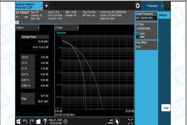
Band5-3MHz-16QAM-20635-15RB#0-PASS
