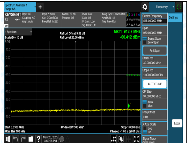
Band2-15MHz-QPSK-18900-1RB#0-30-1000-PASS
