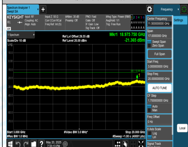
Band2-20MHz-QPSK-18700-1RB#0-3000~20000-PASS
