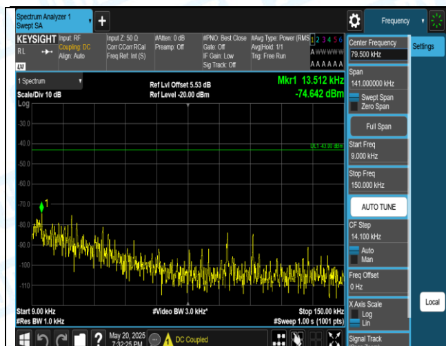
Band2-20MHz-QPSK-18700-1RB#0-0.009~0.15-PASS
