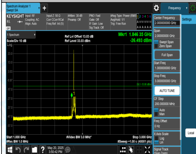
Band2-15MHz-QPSK-18900-1RB#0-1000-3000-PASS
