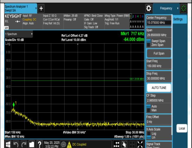
Band2-15MHz-QPSK-19125-1RB#0-0.15-30-PASS
