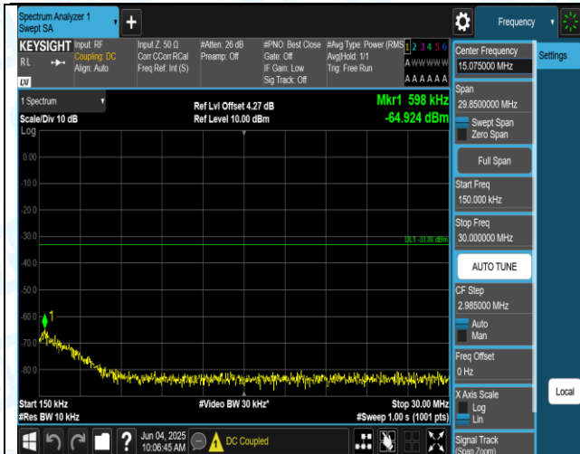
Band2-10MHz-QPSK-18900-1RB#0-0.15-30-PASS
