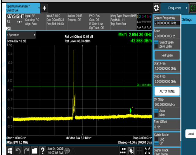
Band2-10MHz-QPSK-18900-1RB#0-1000-3000-PASS
