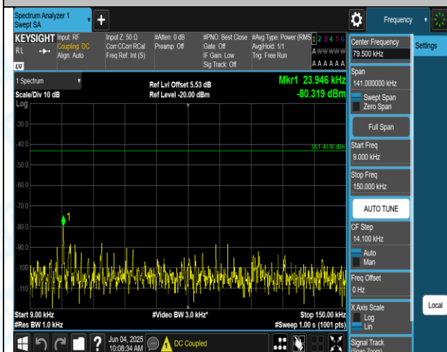
Band2-10MHz-QPSK-19150-1RB#0-0.009-0.15-PASS
