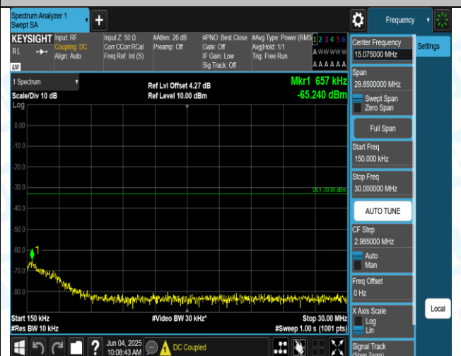
Band2-10MHz-QPSK-19150-1RB#0-0.15-30-PASS
