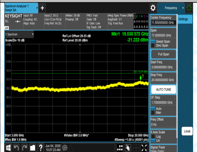
Band2-10MHz-QPSK-18900-1RB#0-3000-20000-PASS
