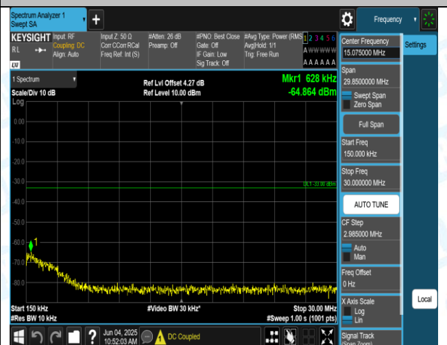
Band2-1.4MHz-QPSK-19193-1RB#0-0.15-30-PASS
