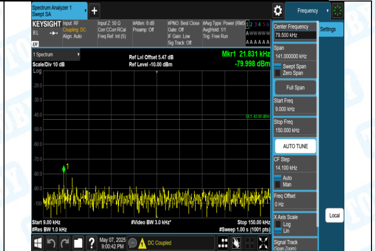
Band2-9538-4-0.009-0.15MHz-PASS
