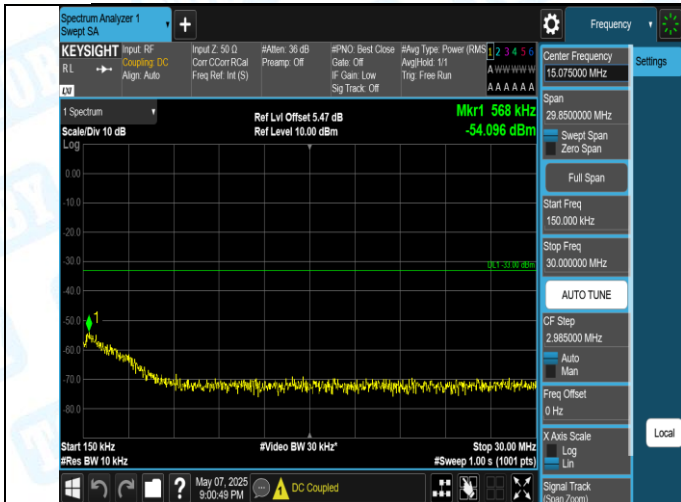
Band2-9538-4-0.15-30MHz-PASS
