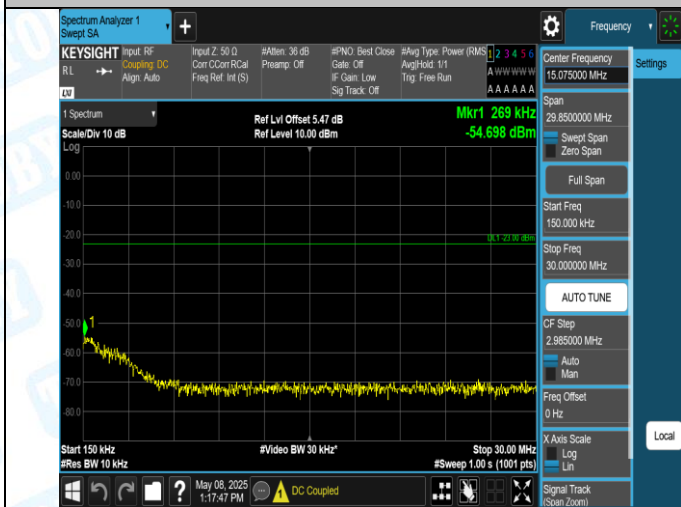
Band5-4132-4-0.15~30MHz-PASS
