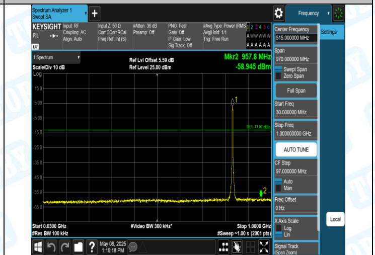
Band5-4182-4-30~1000MHz-PASS
