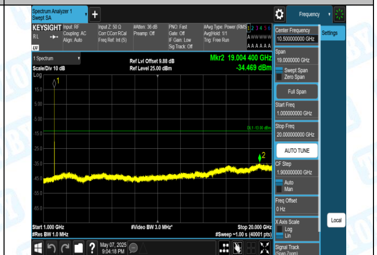
Band2-9538-5-1000~20000MHz-PASS
