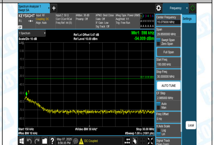
Band2-9538-3-0.15~30MHz-PASS
