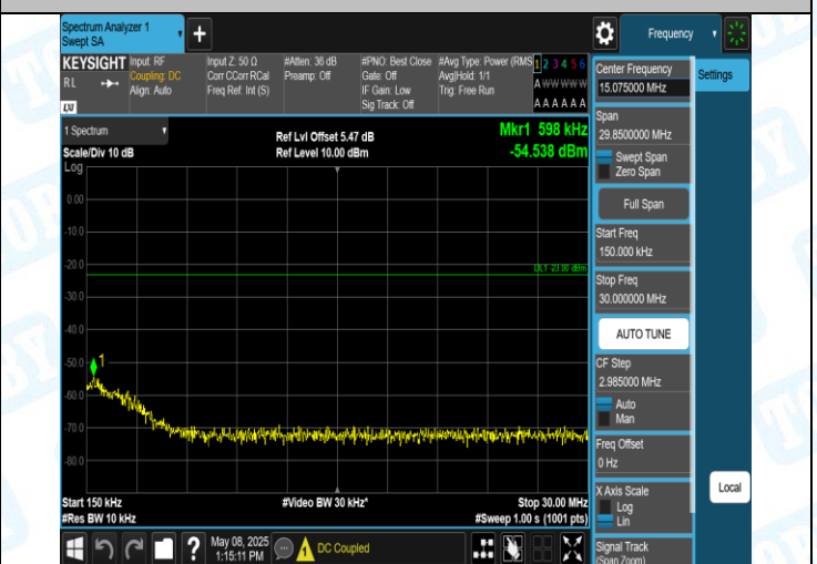
Band5-4182-3-0.15~30MHz-PASS
