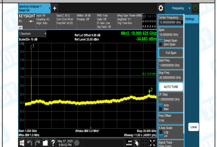
Band2-9538-3-1000~20000MHz-PASS
