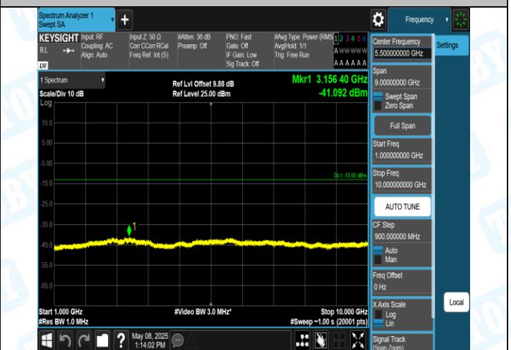
Band5-4132-3-1000~10000MHz-PASS
