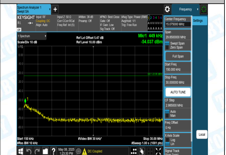
Band5-4182-5-0.15~30MHz-PASS
