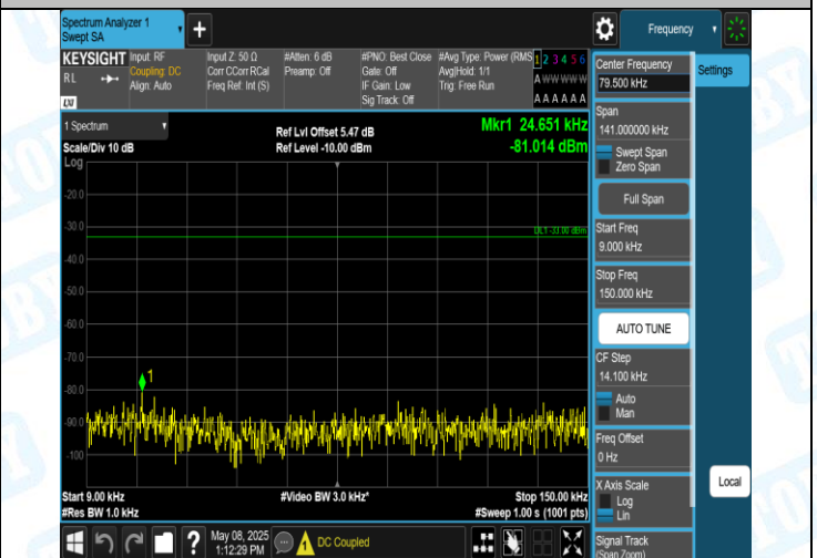
Band5-4233-2-0.009~0.15MHz-PASS
