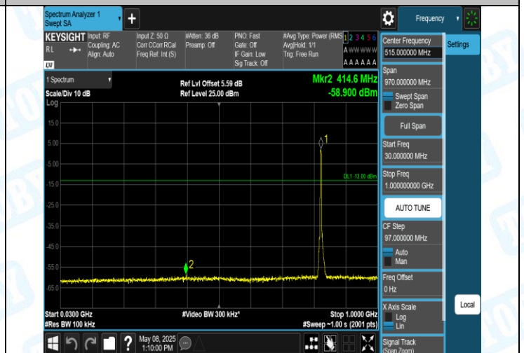
Band5-4132-2-30~1000MHz-PASS
