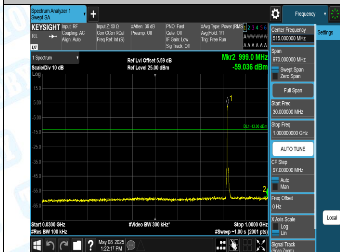
Band5-4132-5-30~1000MHz-PASS
