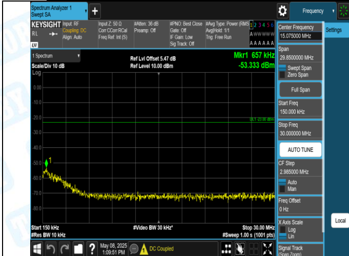
Band5-4132-2-0.15~30MHz-PASS
