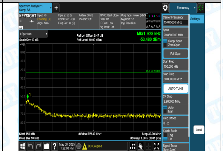
Band5-4132-5-0.15~30MHz-PASS
