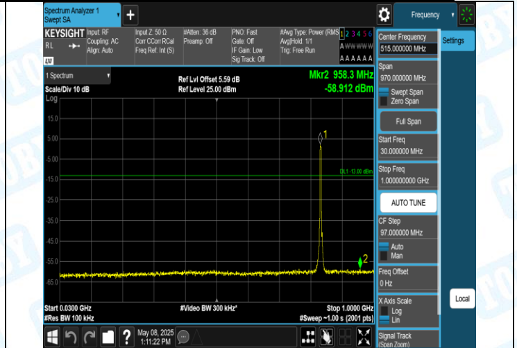
Band5-4182-2-30~1000MHz-PASS
