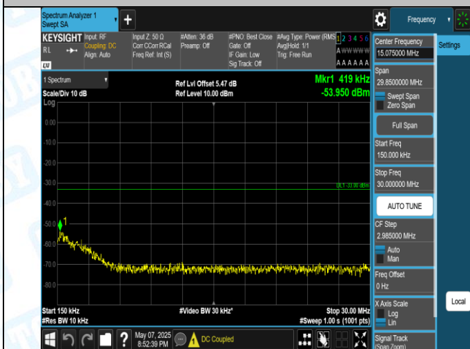
Band2-9538-2-0.15~30MHz-PASS
