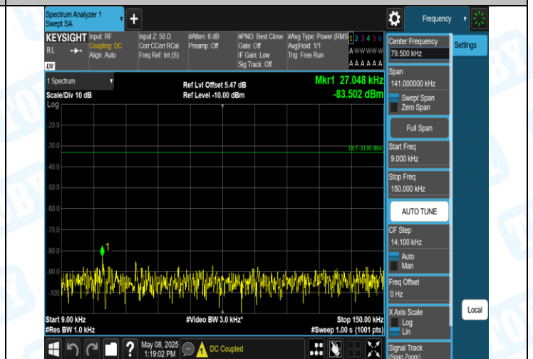
Band5-4182-4-0.009~0.15MHz-PASS
