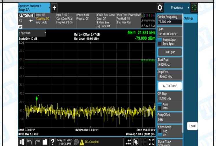
Band5-4182-2-0.009~0.15MHz-PASS
