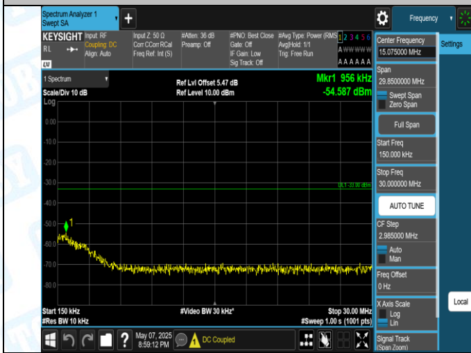
Band2-9400-4-0.15-30MHz-PASS
