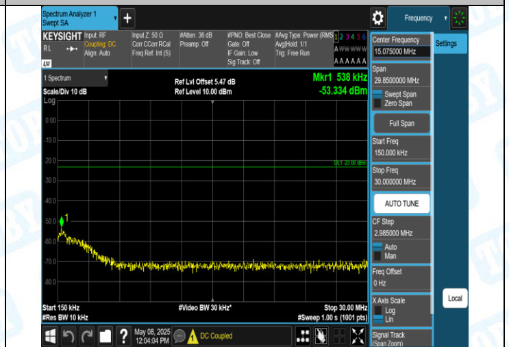
Band5-4233-4-0.15~30MHz-PASS
