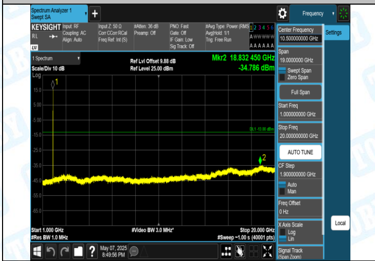
Band2-9262-2-1000~20000MHz-PASS
