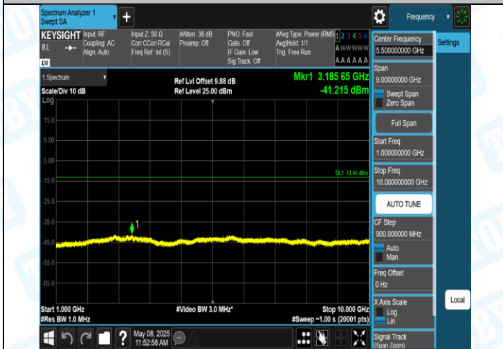
Band5-4233-1-1000~10000MHz-PASS
