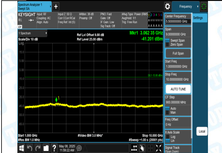
Band5-4182-3-1000-10000MHz-PASS
