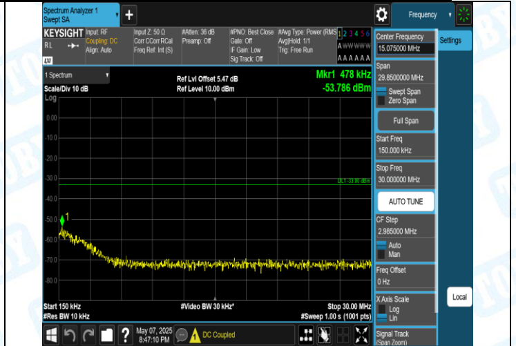
Band2-9400-1-0.15-30MHz-PASS
