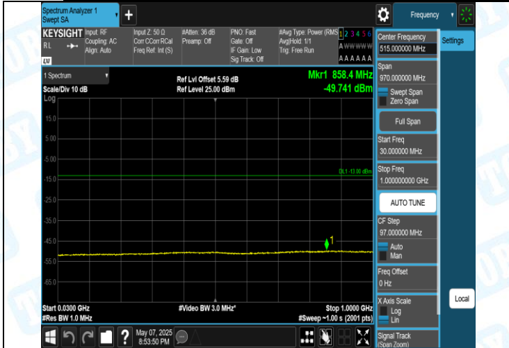
Band2-9262-3-30~1000MHz-PASS
