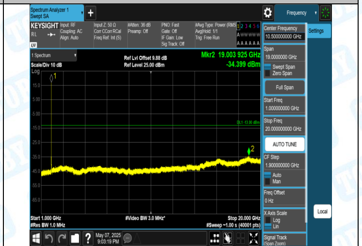
Band2-9400-5-1000~20000MHz-PASS
