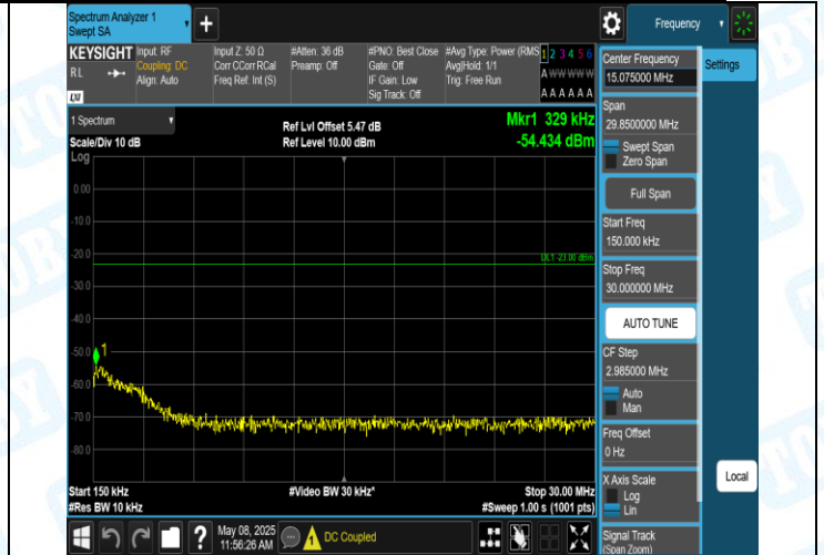
Band5-4233-2-0.15~30MHz-PASS
