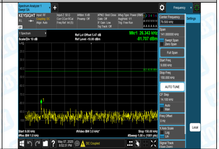
Band2-9538-2-0.009~0.15MHz-PASS
