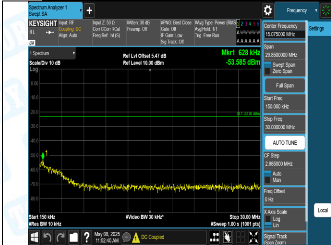
Band5-4233-1-0.15~30MHz-PASS
