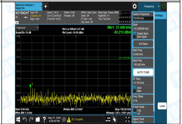
Band2-9400-4-0.009~0.15MHz-PASS
