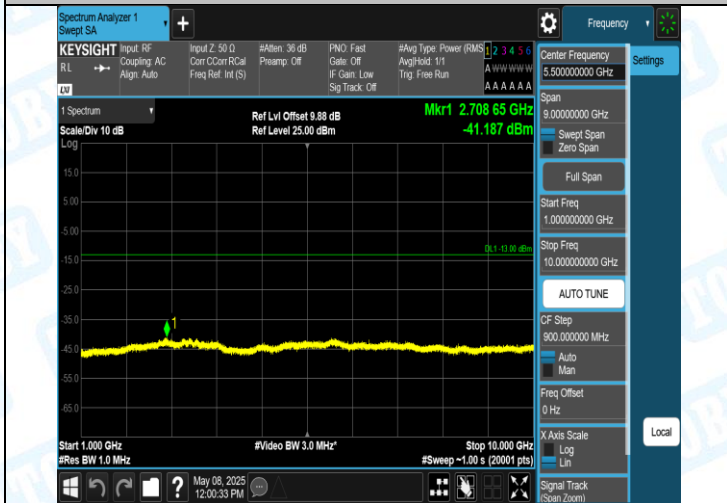
Band5-4233-3-1000~10000MHz-PASS
