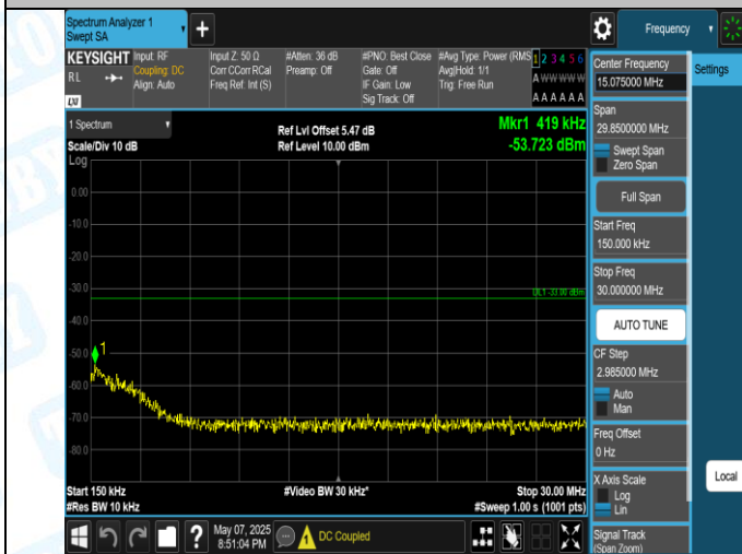
Band2-9400-2-0.15-30MHz-PASS
