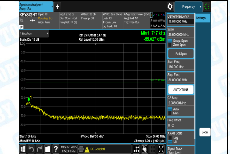
Band2-9262-3-0.15-30MHz-PASS
