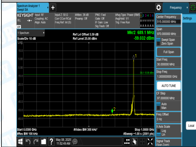
Band5-4233-1-30~1000MHz-PASS
