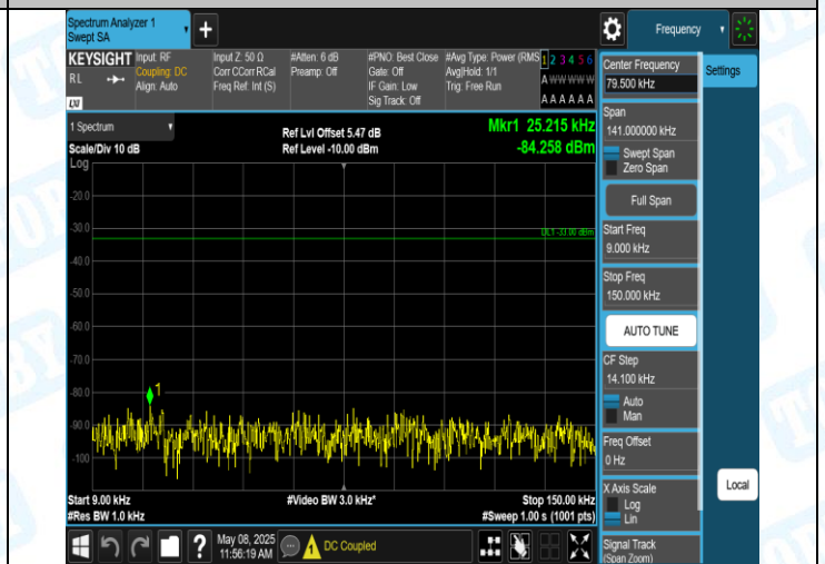
Band5-4233-2-0.009-0.15MHz-PASS
