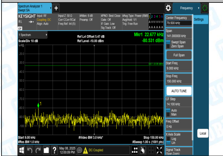
Band5-4233-3-0.009-0.15MHz-PASS
