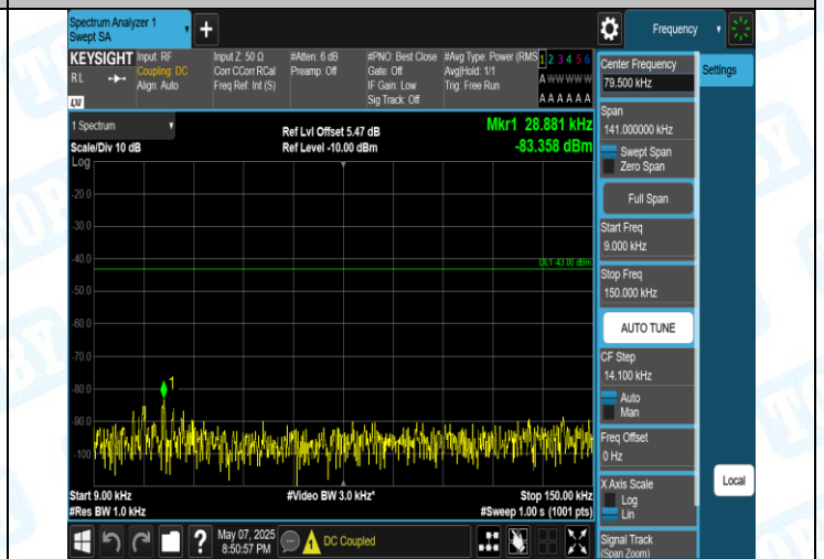
Band2-9400-2-0.009~0.15MHz-PASS
