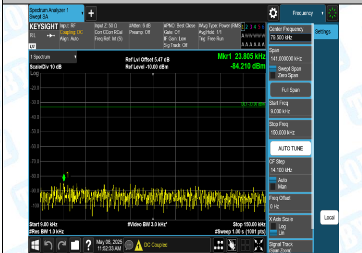
Band5-4233-1-0.009-0.15MHz-PASS
