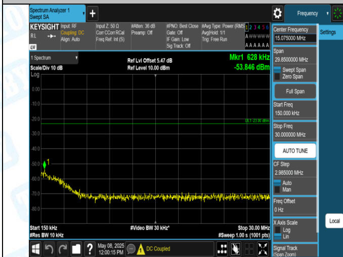
Band5-4233-3-0.15~30MHz-PASS
