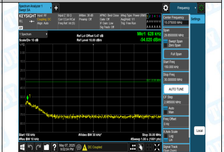
Band2-9262-5-0.15-30MHz-PASS
