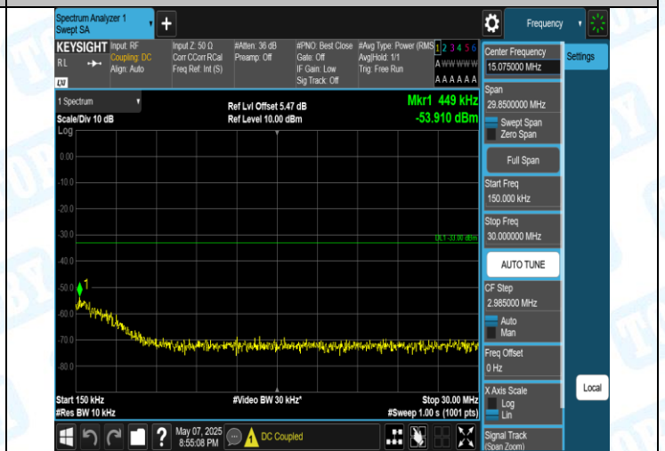
Band2-9400-3-0.15-30MHz-PASS
