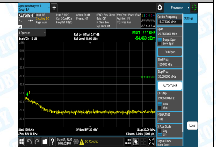
Band2-9400-5-0.15-30MHz-PASS
