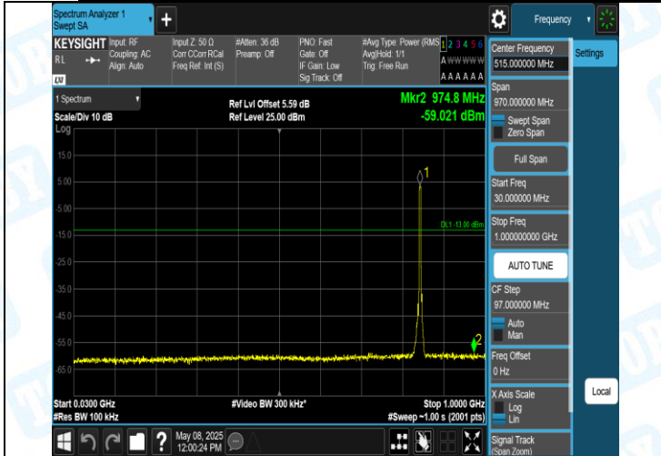
Band5-4233-3-30~1000MHz-PASS
