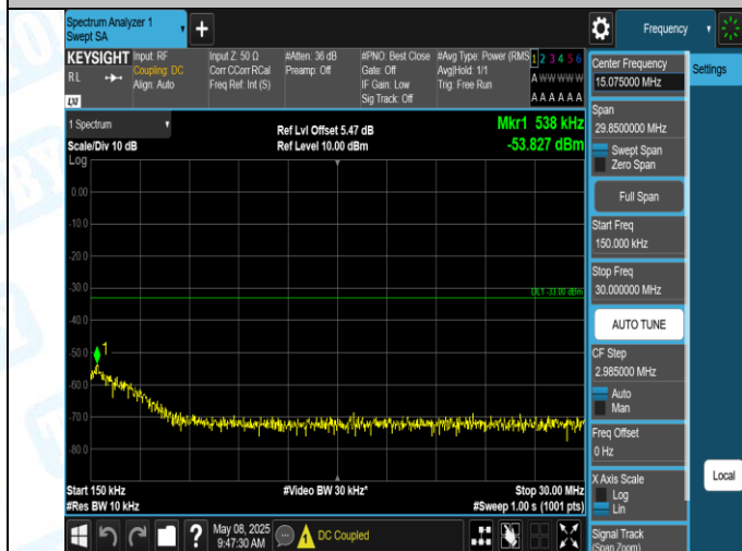
Band2-9538-3-0.15~30MHz-PASS
