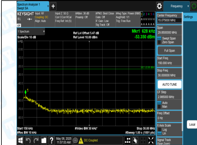
Band5-4132-3-0.15~30MHz-PASS
