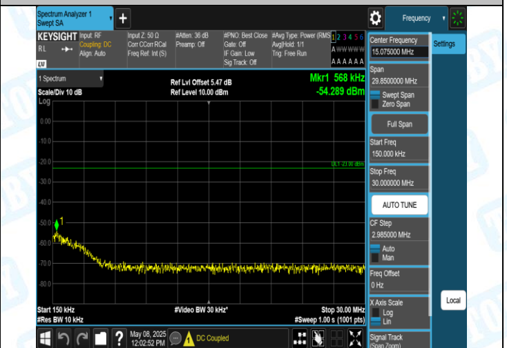
Band5-4182-4-0.15~30MHz-PASS
