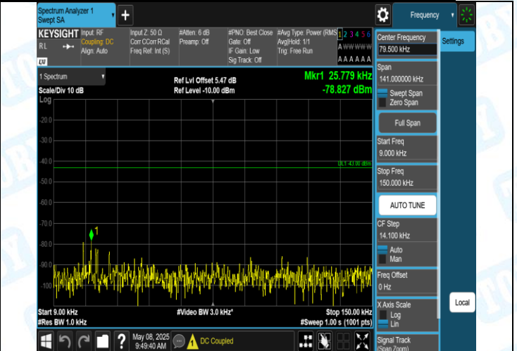
Band2-9400-4-0.009-0.15MHz-PASS
