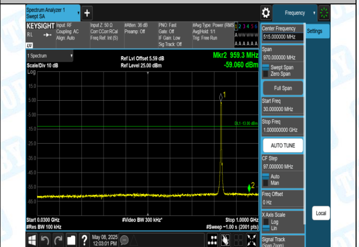
Band5-4182-4-30~1000MHz-PASS
