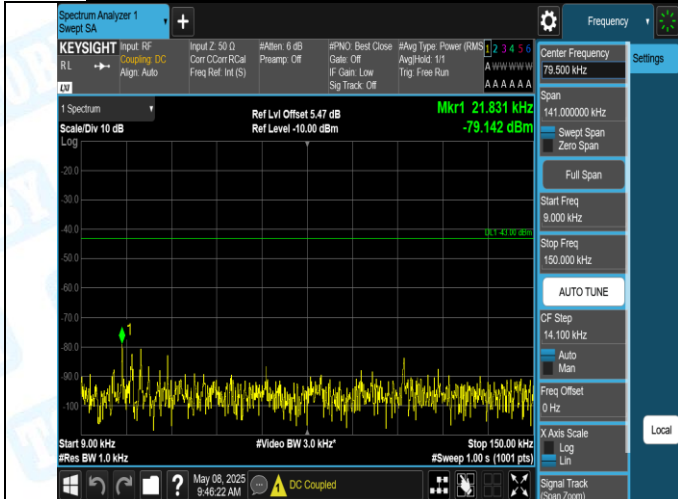
Band2-9400-3-0.009-0.15MHz-PASS
