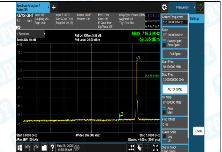
Band5-4182-2-30~1000MHz-PASS
