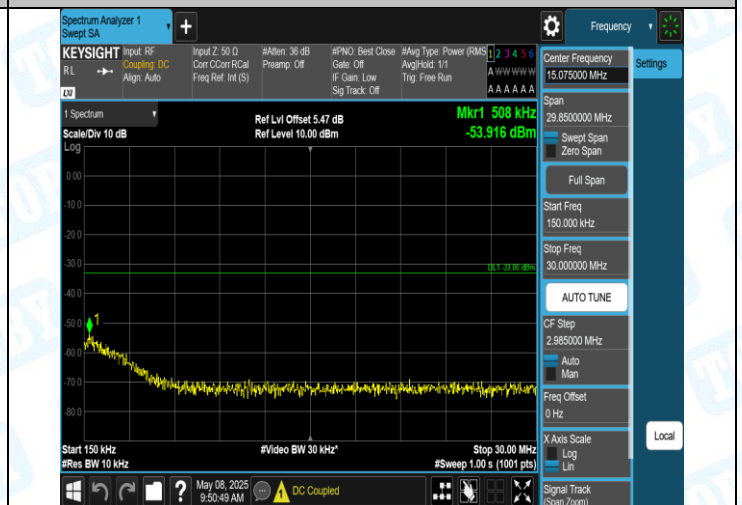
Band2-9538-4-0.15~30MHz-PASS
