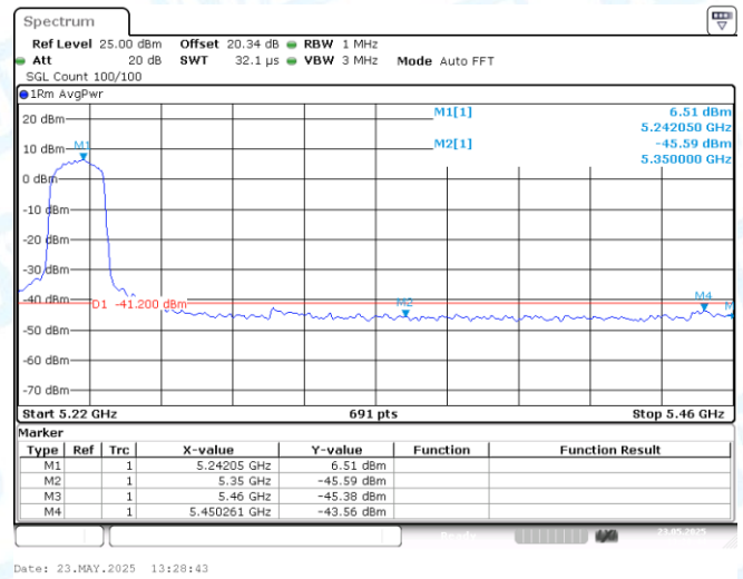
11AC20SISO-Ant1-5240-PASS
