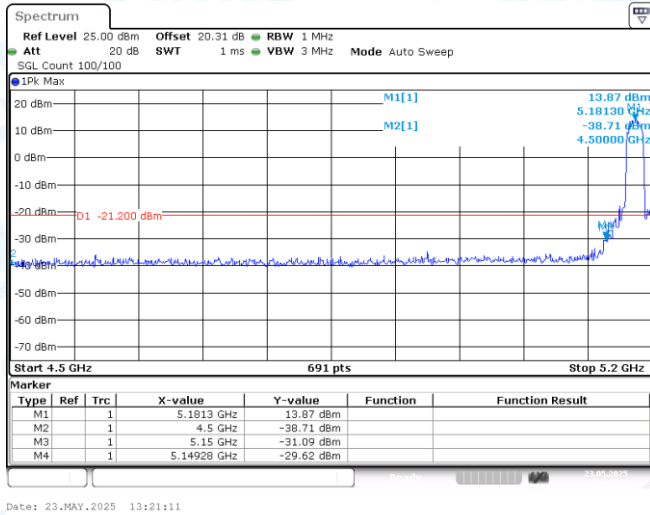
11AC20SISO-Ant1-5180-PASS
