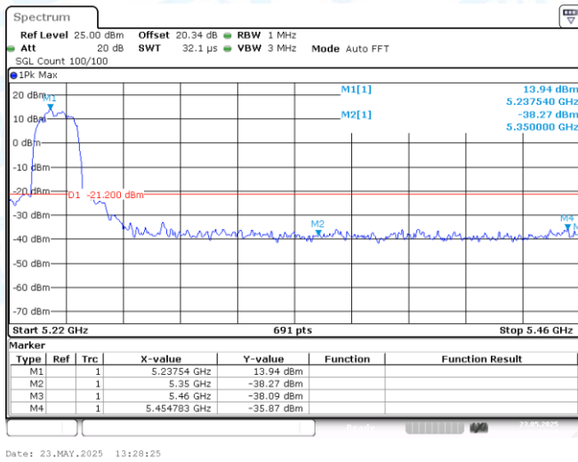
11AC20SISO-Ant1-5240-PASS
