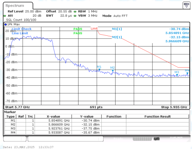
11AC20SISO-Ant1-5825-PASS
