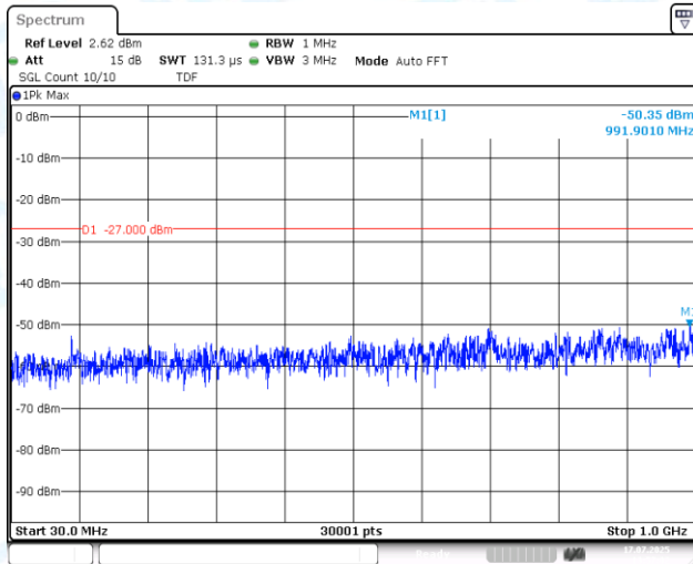
11AC40SISO-Ant1-5795-30~1000-PASS
