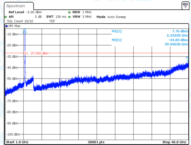
11AC40SISO-Ant1-5190-1000~40000-PASS
