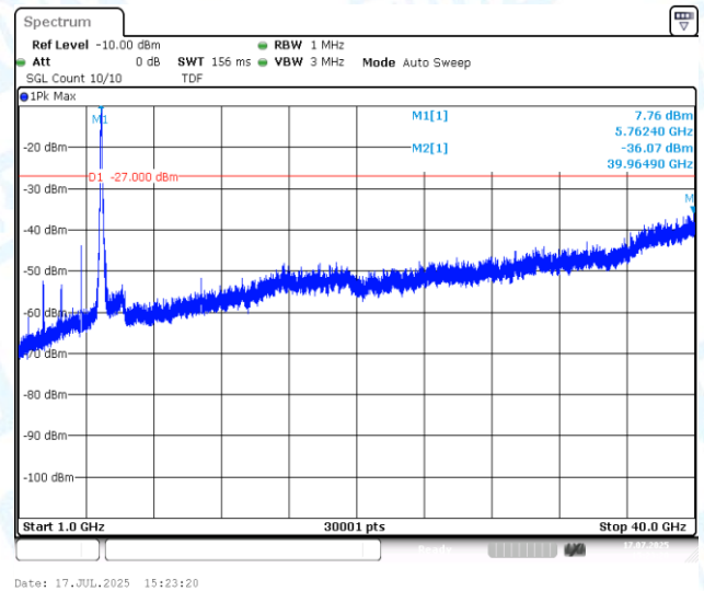
11N40SISO-Ant1-5755-1000~40000-PASS
