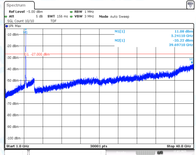
11AC20SISO-Ant1-5240-1000~40000-PASS
