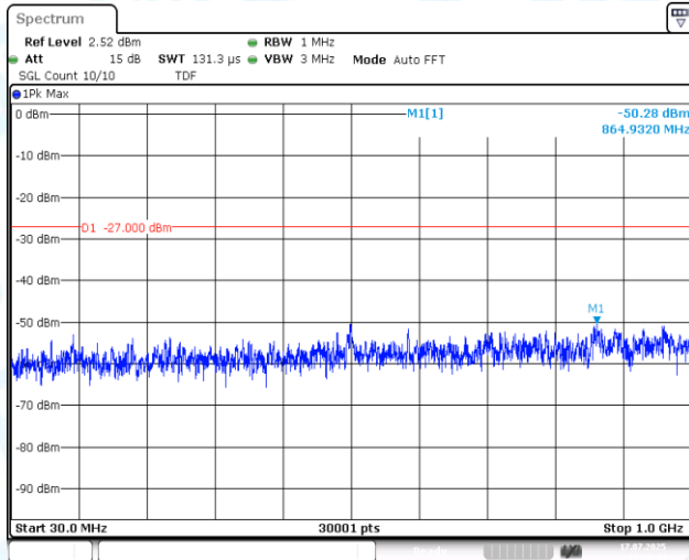
11AC20SISO-Ant1-5240-30~1000-PASS
