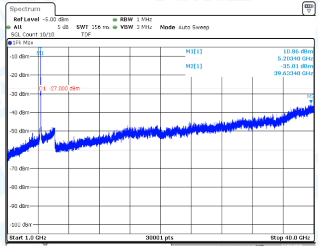
11AC20SISO-Ant1-5180-1000~40000-PASS
