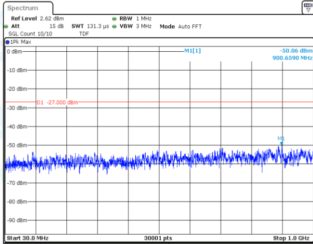
11AC20SISO-Ant1-5825-30~1000-PASS
