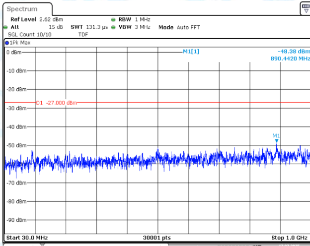
11AC20SISO-Ant1-5180-30~1000-PASS
