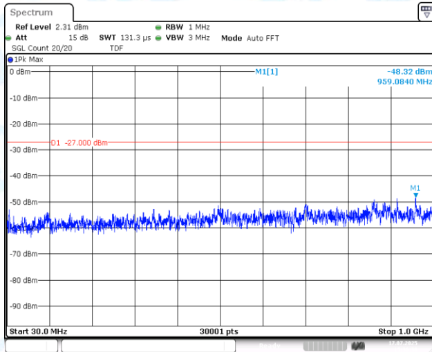
11AC20SISO-Ant1-5745-30~1000-PASS
