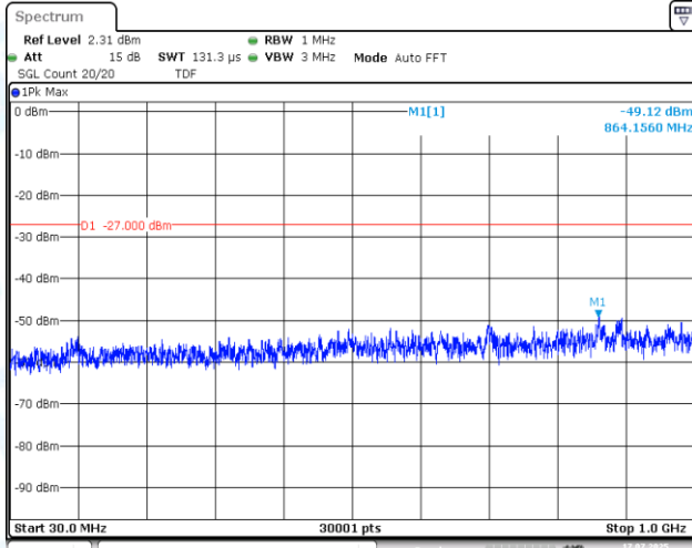
11N40SISO-Ant1-5795-30~1000-PASS
