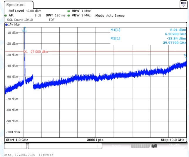
11N40SISO-Ant1-5230-1000~40000-PASS
