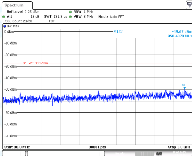
11AC40SISO-Ant1-5755-30~1000-PASS
