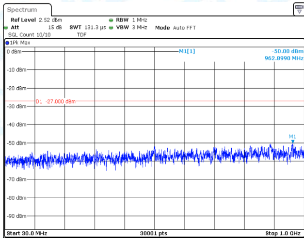
11AC40SISO-Ant1-5190-30~1000-PASS
