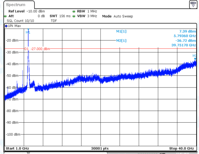
11N40SISO-Ant1-5795-1000~40000-PASS
