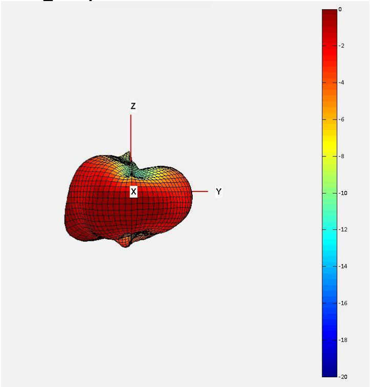
2500MHz H&V_ Y-Z plane
