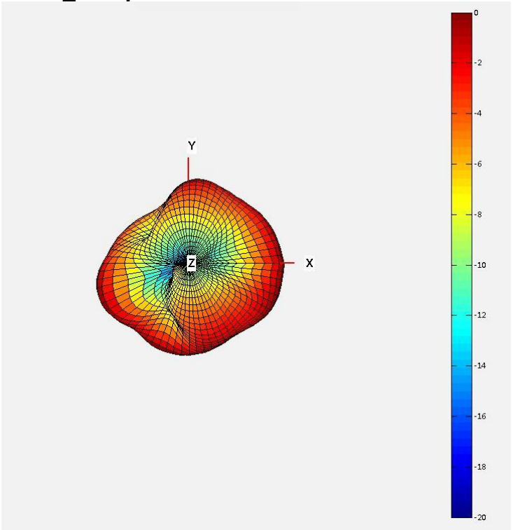
2400MHz H&V_ X-Y plane
