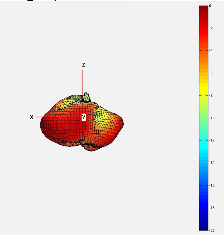
2450MHz H&V_ X-Z plane
