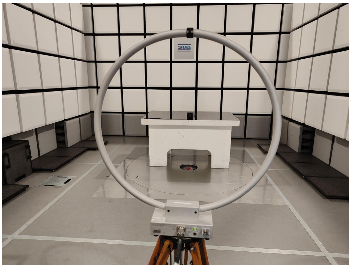
Figure 1: Spurious emission 90 kHz-30 MHz
