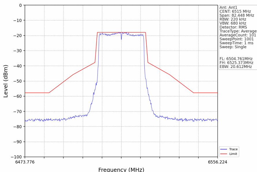
802.11ax(HEW20)_HCH_6515MHz_RU242_Left_Ant1_NTNV
