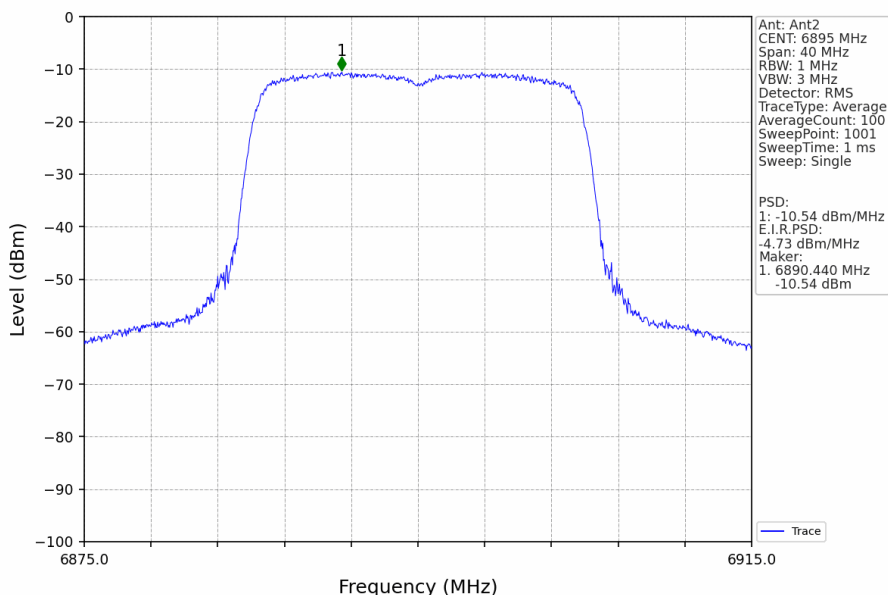
802.11ax(HEW20)_LCH_6895MHz_RU242_Left_MIMO_NTNV
