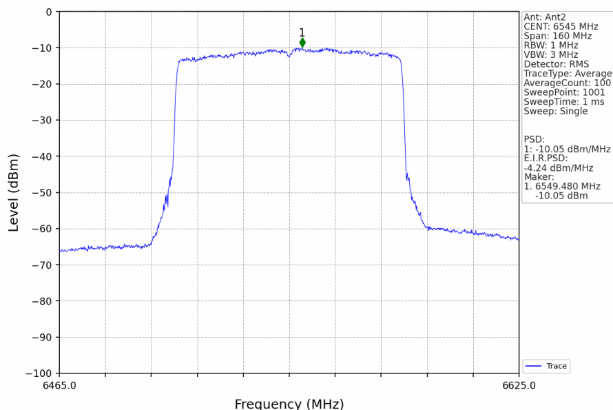
802.11ax(HEW80)_HCH_6545MHz_RU996_Left_MIMO_NTNV
