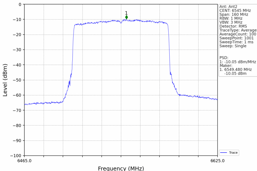
802.11ax(HEW80)_HCH_6545MHz_RU996_Left_MIMO_NTNV
