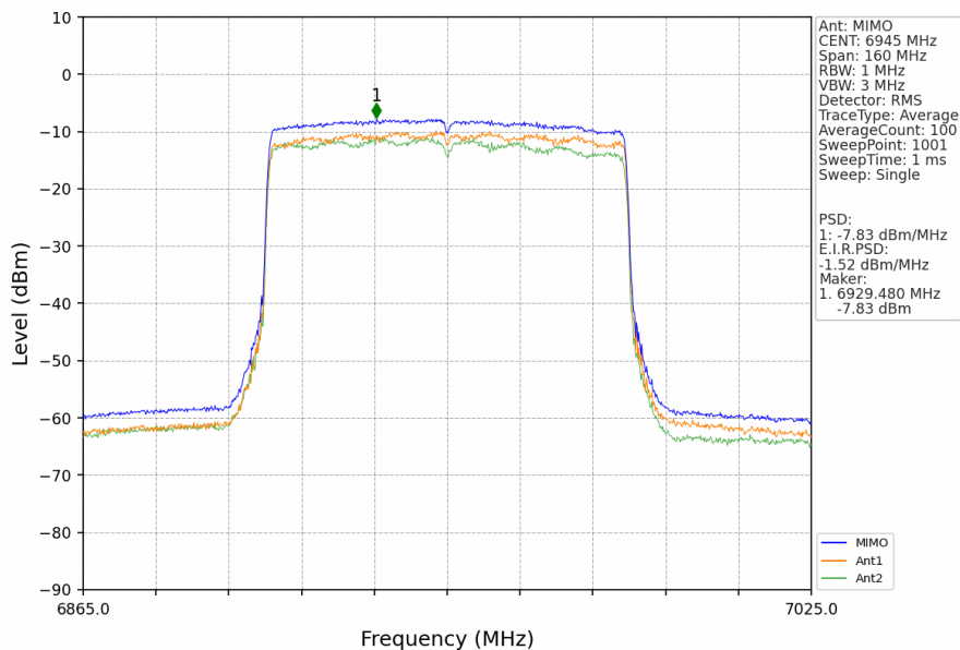
802.11ax(HEW80)_LCH_6945MHz_RU996_Left_MIMO_NTNV
