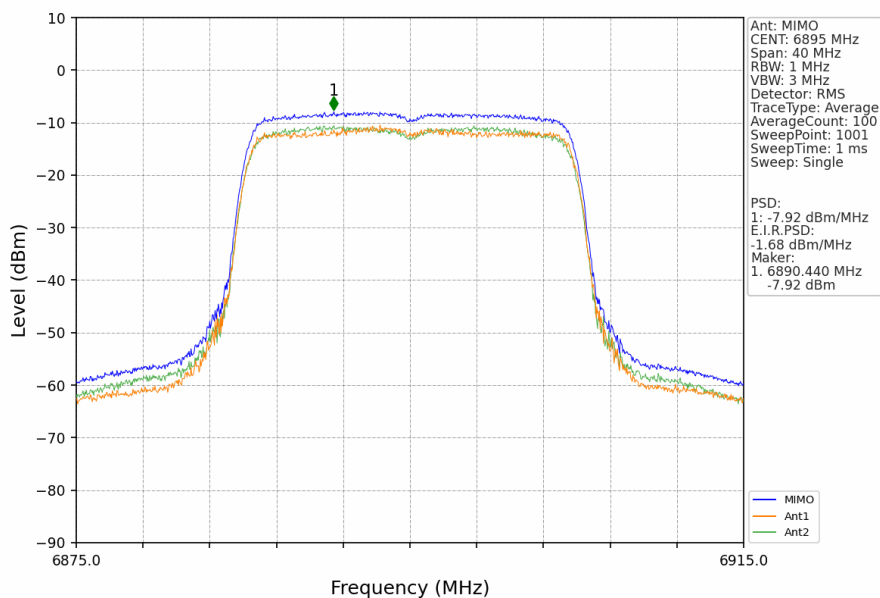
802.11ax(HEW20)_LCH_6895MHz_RU242_Left_MIMO_NTNV
