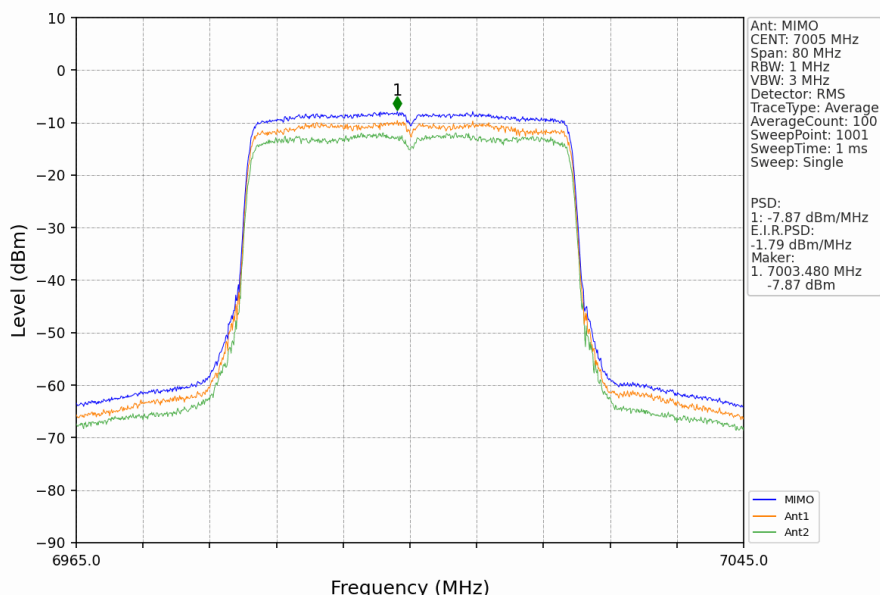
802.11ax(HEW40)_MCH_7005MHz_RU484_Left_MIMO_NTNV
