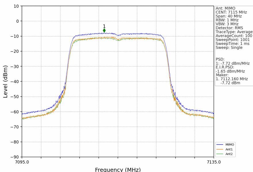
802.11ax(HEW20)_HCH_7115MHz_RU242_Left_MIMO_NTNV
