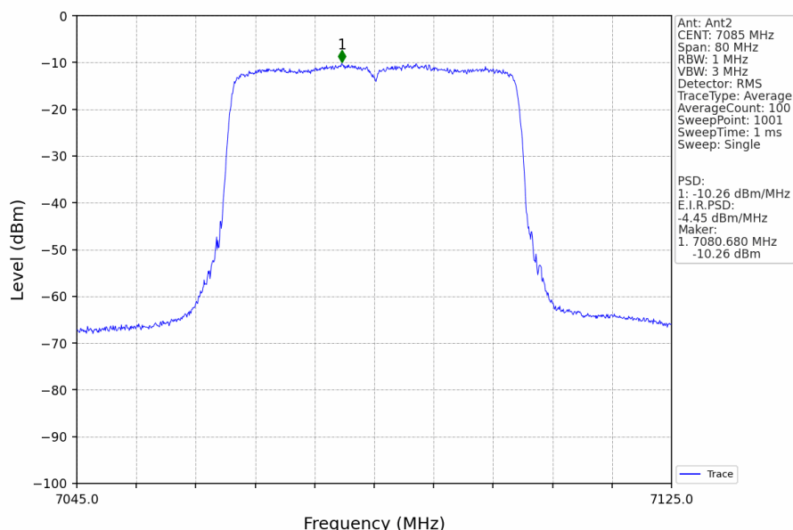
802.11ax(HEW40)_HCH_7085MHz_RU484_Left_Ant2_NTNV
