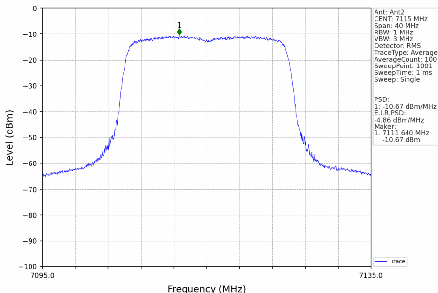
802.11ax(HEW20)_HCH_7115MHz_RU242_Left_MIMO_NTNV
