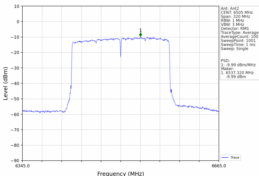
802.11ax(HEW160)_HCH_6505MHz_2xRU996_Left_Ant2_NTNV
