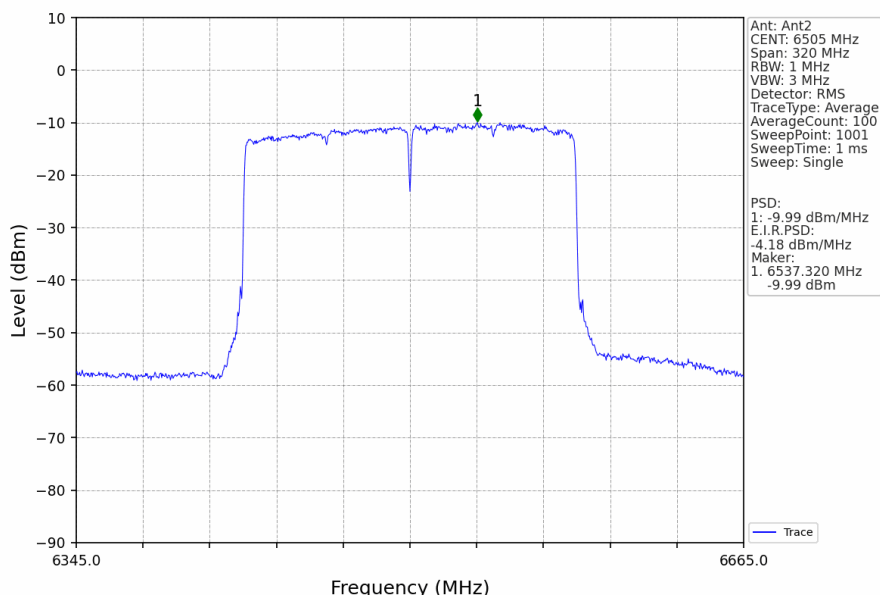
802.11ax(HEW160)_HCH_6505MHz_2xRU996_Left_Ant2_NTNV
