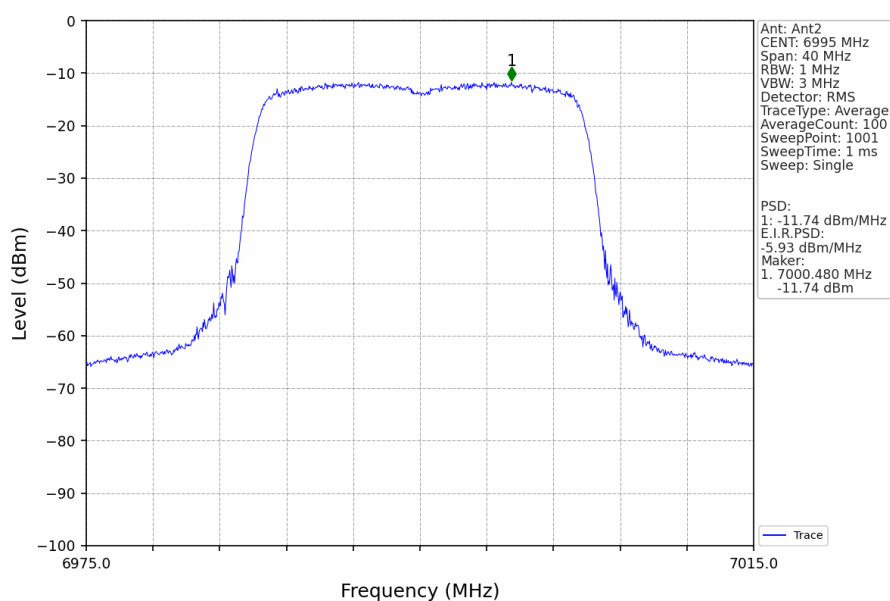
802.11ax(HEW20)_MCH_6995MHz_RU242_Left_Ant2_NTNV
