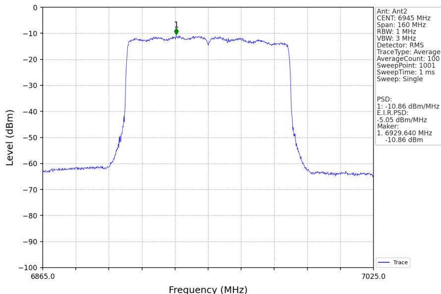
802.11ax(HEW80)_LCH_6945MHz_RU996_Left_MIMO_NTNV
