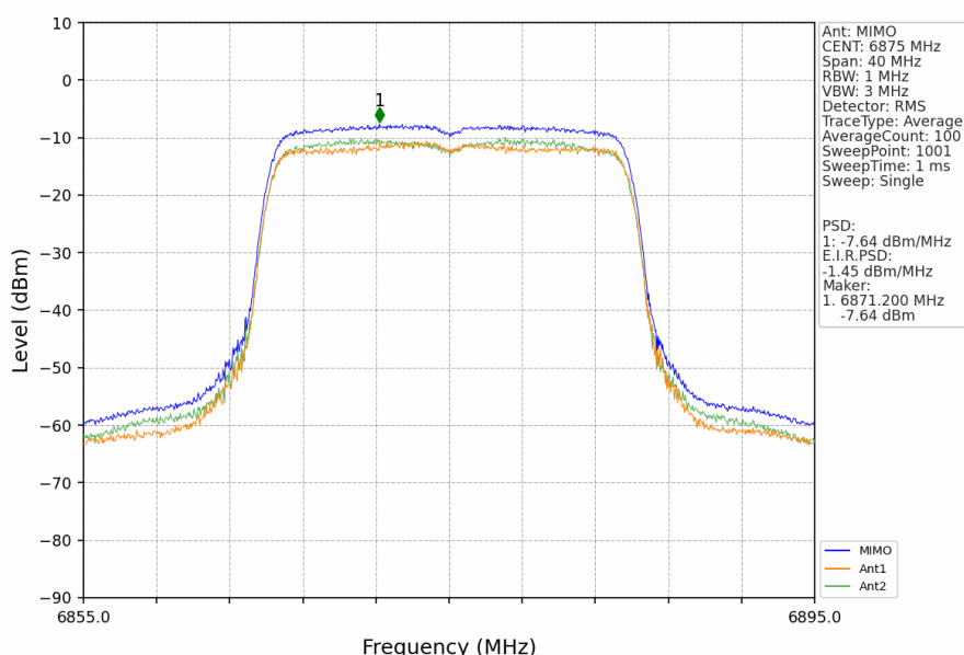
802.11ax(HEW20)_HCH_6875MHz_RU242_Left_MIMO_NTNV
