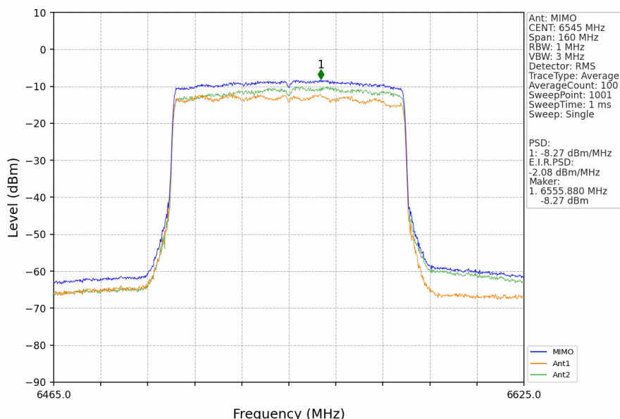
802.11ax(HEW80)_HCH_6545MHz_RU996_Left_MIMO_NTNV
