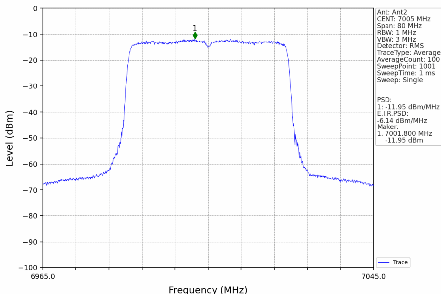
802.11ax(HEW40)_MCH_7005MHz_RU484_Left_MIMO_NTNV
