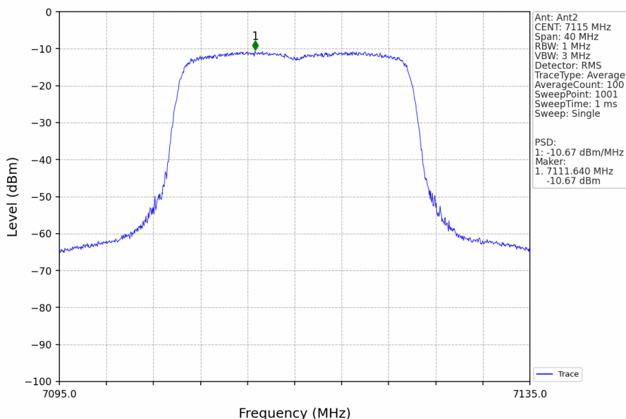
802.11ax(HEW20)_HCH_7115MHz_RU242_Left_MIMO_NTNV
