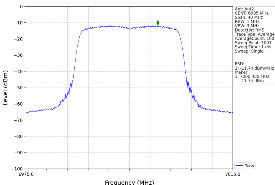
802.11ax(HEW20)_MCH_6995MHz_RU242_Left_Ant2_NTNV
