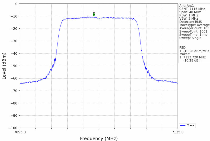
802.11ax(HEW20)_HCH_7115MHz_RU242_Left_Ant1_NTNV
