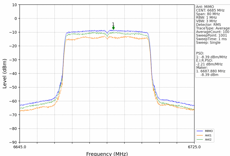
802.11ax(HEW40)_MCH_6685MHz_RU484_Left_MIMO_NTNV
