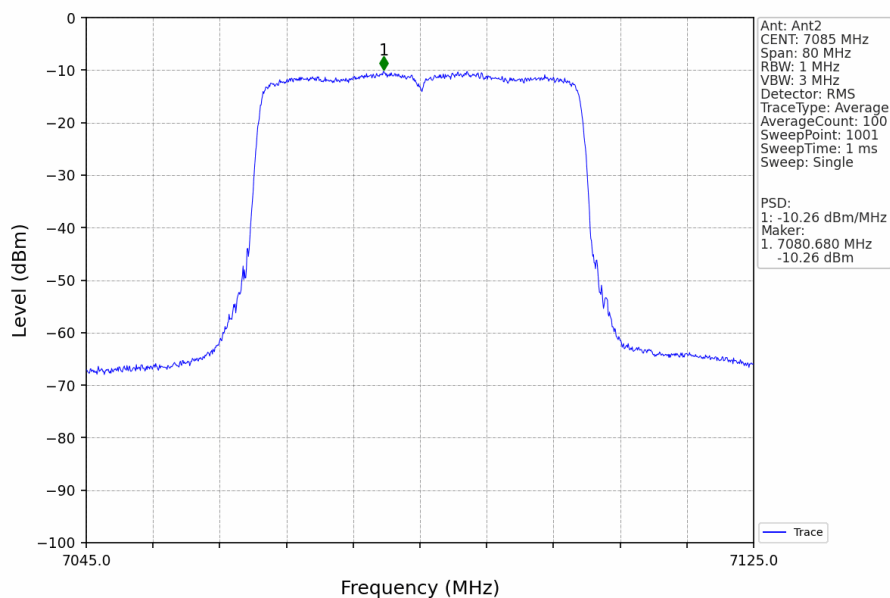
802.11ax(HEW40)_HCH_7085MHz_RU484_Left_Ant2_NTNV
