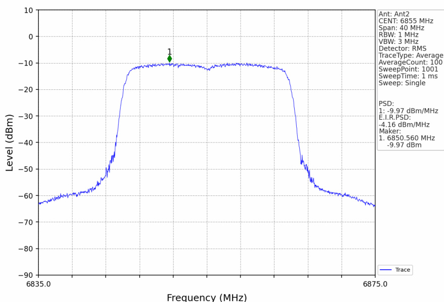
802.11ax(HEW20)_HCH_6855MHz_RU242_Left_MIMO_NTNV
