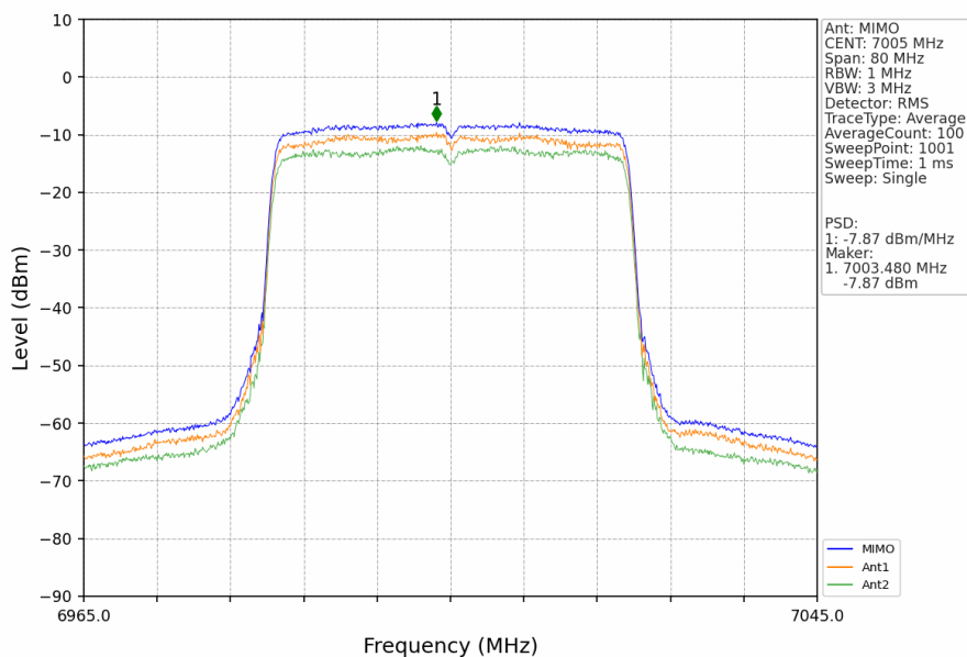
802.11ax(HEW40)_MCH_7005MHz_RU484_Left_MIMO_NTNV
