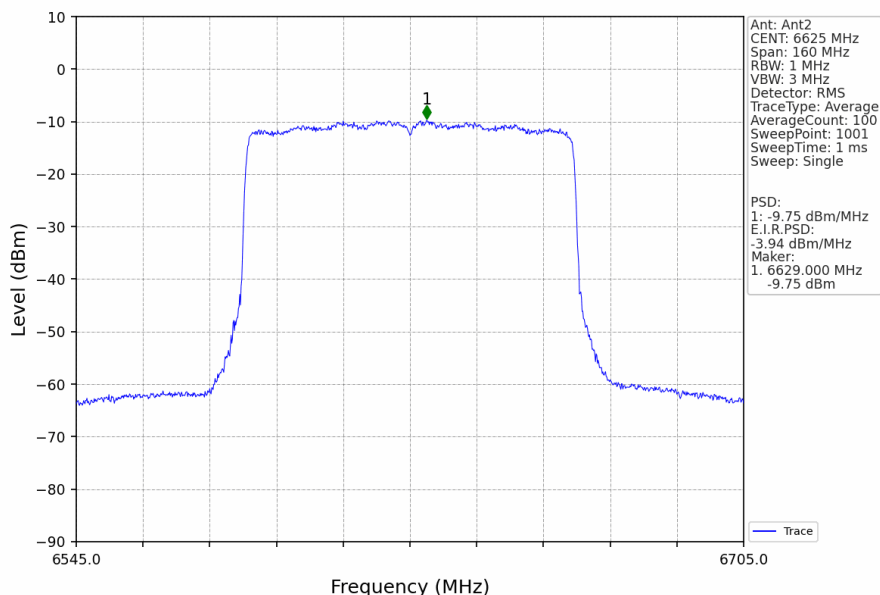
802.11ax(HEW80)_LCH_6625MHz_RU996_Left_MIMO_NTNV
