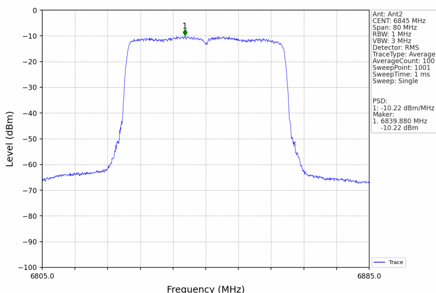
802.11ax(HEW40)_HCH_6845MHz_RU484_Left_Ant2_NTNV
