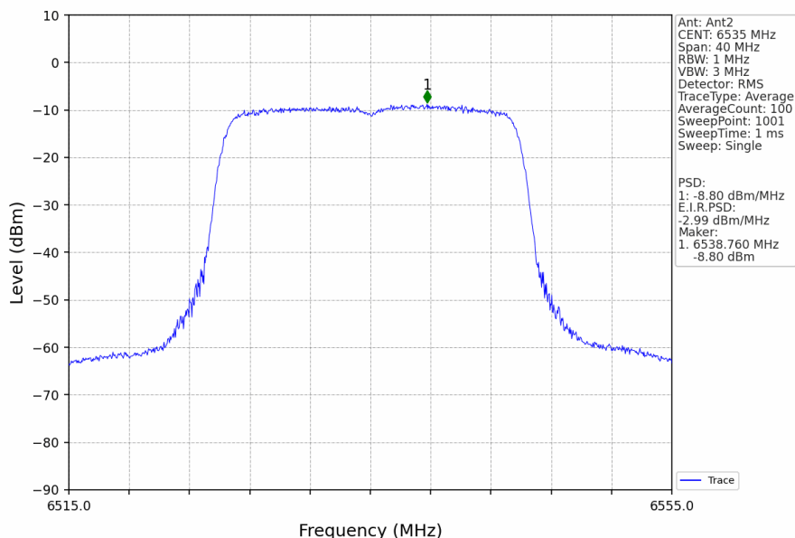
802.11ax(HEW20)_LCH_6535MHz_RU242_Left_MIMO_NTNV
