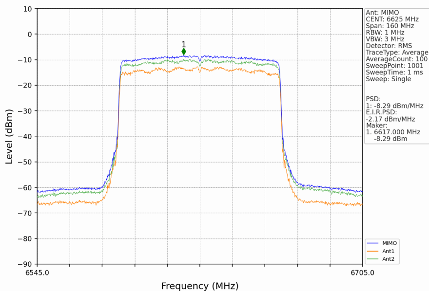
802.11ax(HEW80)_LCH_6625MHz_RU996_Left_MIMO_NTNV
