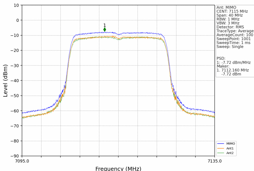
802.11ax(HEW20)_HCH_7115MHz_RU242_Left_MIMO_NTNV
