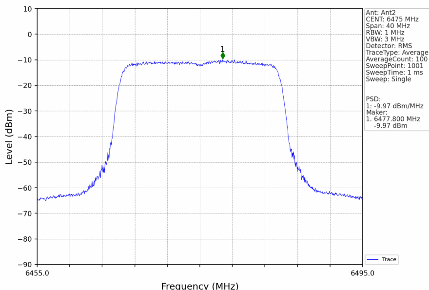
802.11ax(HEW20)_MCH_6475MHz_RU242_Left_Ant2_NTNV
