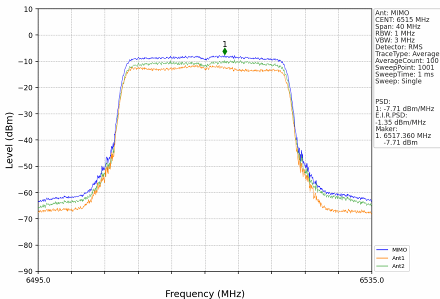
802.11ax(HEW20)_HCH_6515MHz_RU242_Left_MIMO_NTNV
