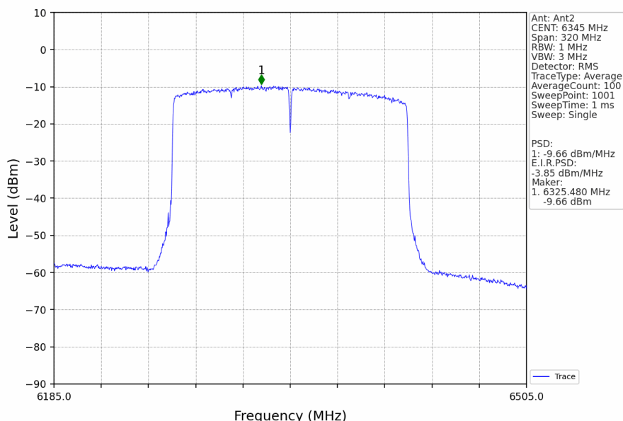
802.11ax(HEW160)_HCH_6345MHz_2xRU996_Left_Ant2_NTNV
