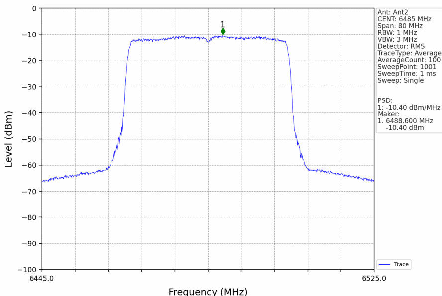
802.11ax(HEW40)_MCH_6485MHz_RU484_Left_MIMO_NTNV
