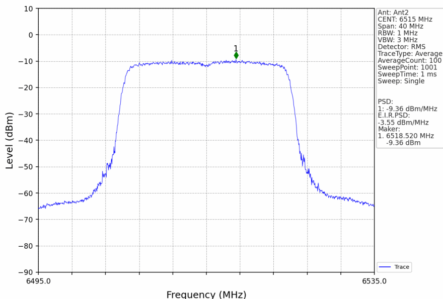
802.11ax(HEW20)_HCH_6515MHz_RU242_Left_MIMO_NTNV
