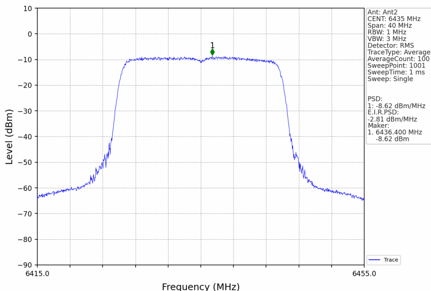
802.11ax(HEW20)_LCH_6435MHz_RU242_Left_MIMO_NTNV
