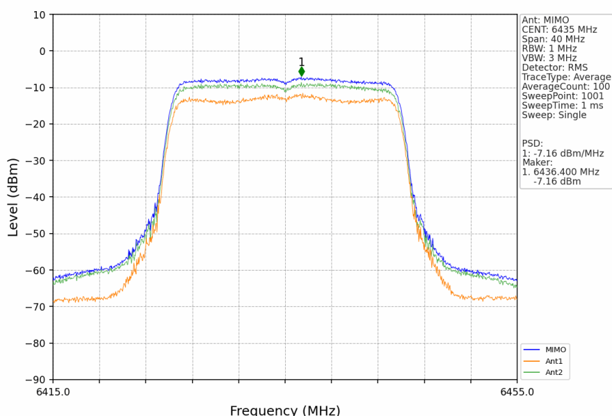
802.11ax(HEW20)_LCH_6435MHz_RU242_Left_MIMO_NTNV
