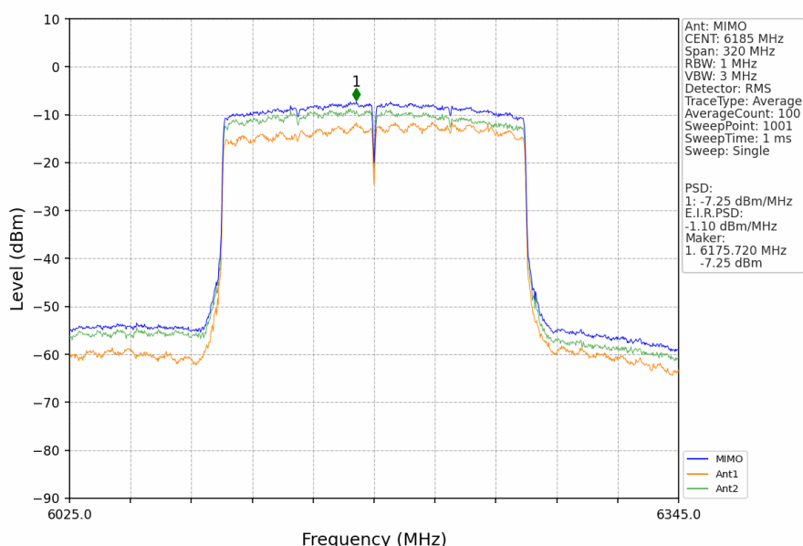
802.11ax(HEW160)_MCH_6185MHz_2xRU996_Left_MIMO_NTNV
