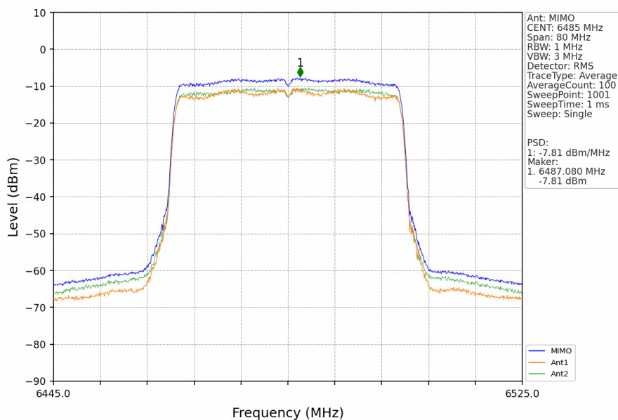
802.11ax(HEW40)_MCH_6485MHz_RU484_Left_MIMO_NTNV
