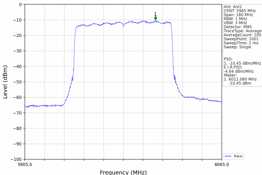
802.11ax(HEW80)_LCH_5985MHz_RU996_Left_MIMO_NTNV
