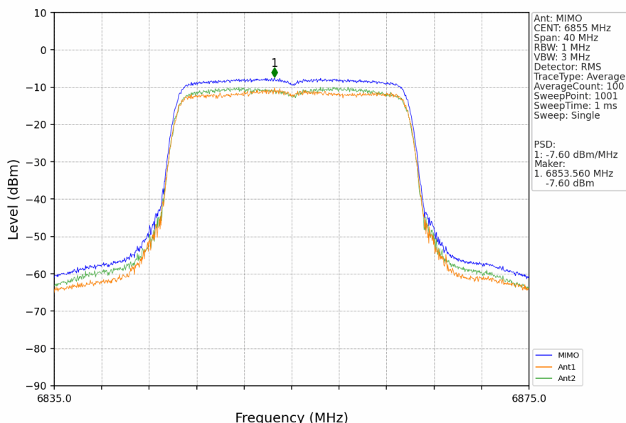
802.11ax(HEW20)_HCH_6855MHz_RU242_Left_MIMO_NTNV
