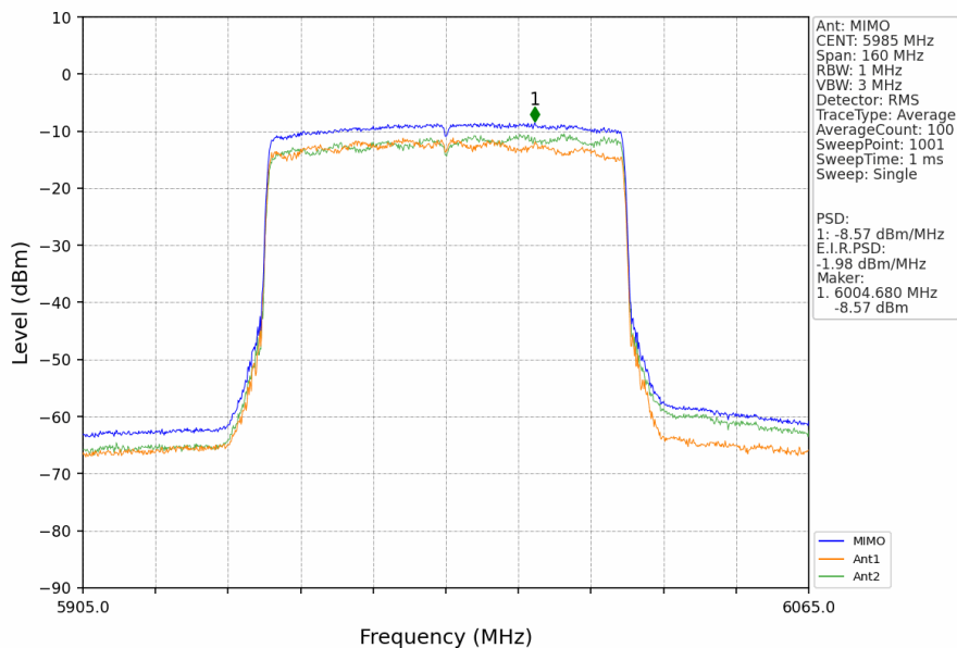
802.11ax(HEW80)_LCH_5985MHz_RU996_Left_MIMO_NTNV
