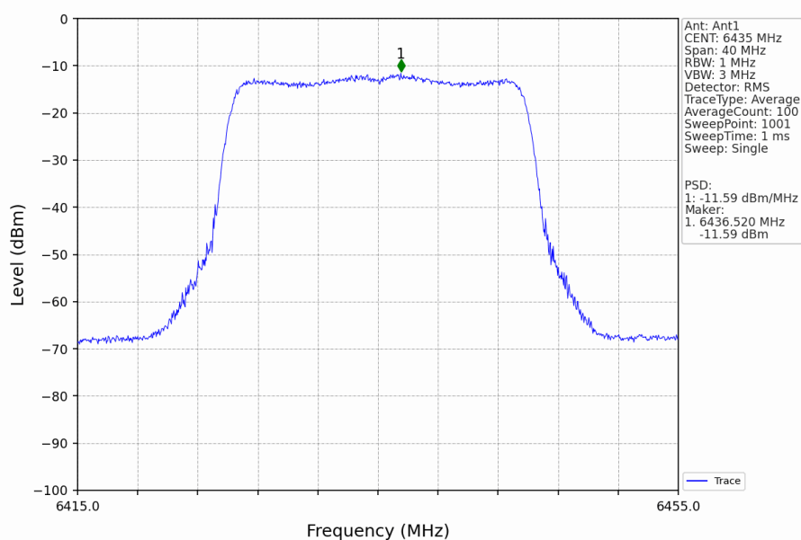
802.11ax(HEW20)_LCH_6435MHz_RU242_Left_Ant1_NTNV
