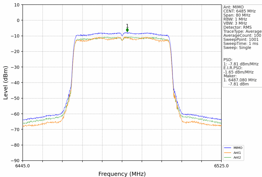
802.11ax(HEW40)_MCH_6485MHz_RU484_Left_MIMO_NTNV
