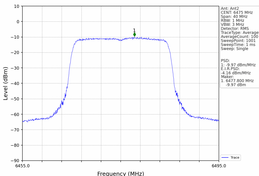
802.11ax(HEW20)_MCH_6475MHz_RU242_Left_Ant2_NTNV
