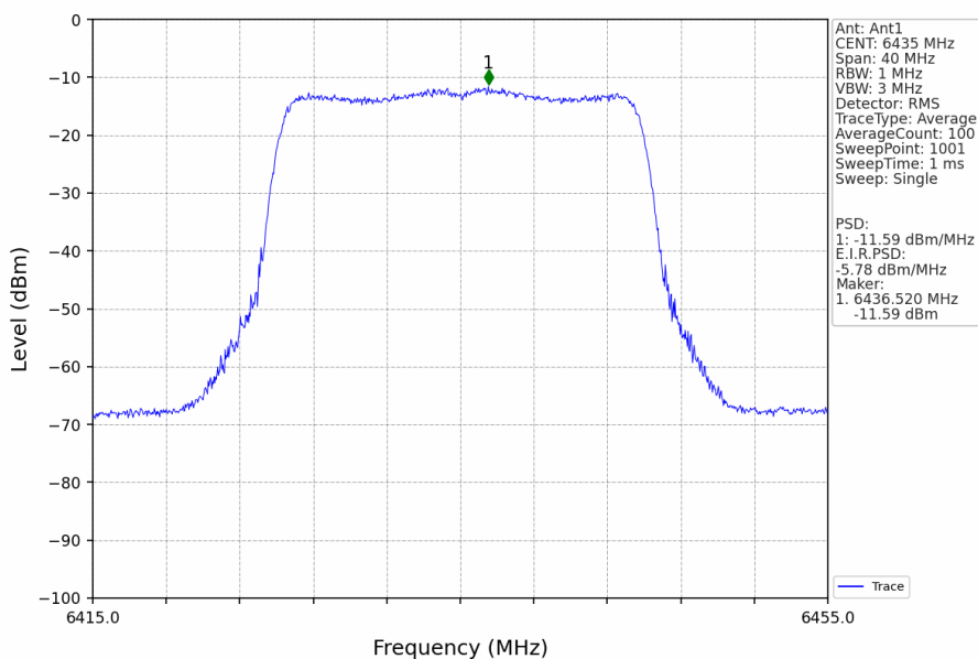
802.11ax(HEW20)_LCH_6435MHz_RU242_Left_Ant1_NTNV
