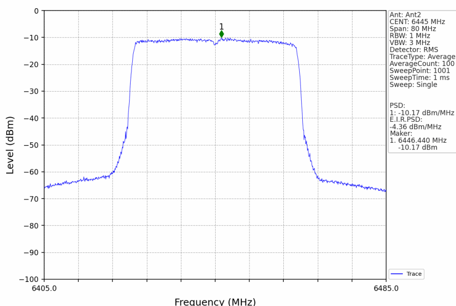
802.11ax(HEW40)_LCH_6445MHz_RU484_Left_Ant2_NTNV
