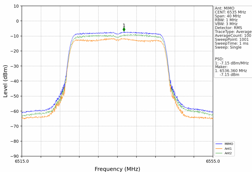
802.11ax(HEW20)_LCH_6535MHz_RU242_Left_MIMO_NTNV
