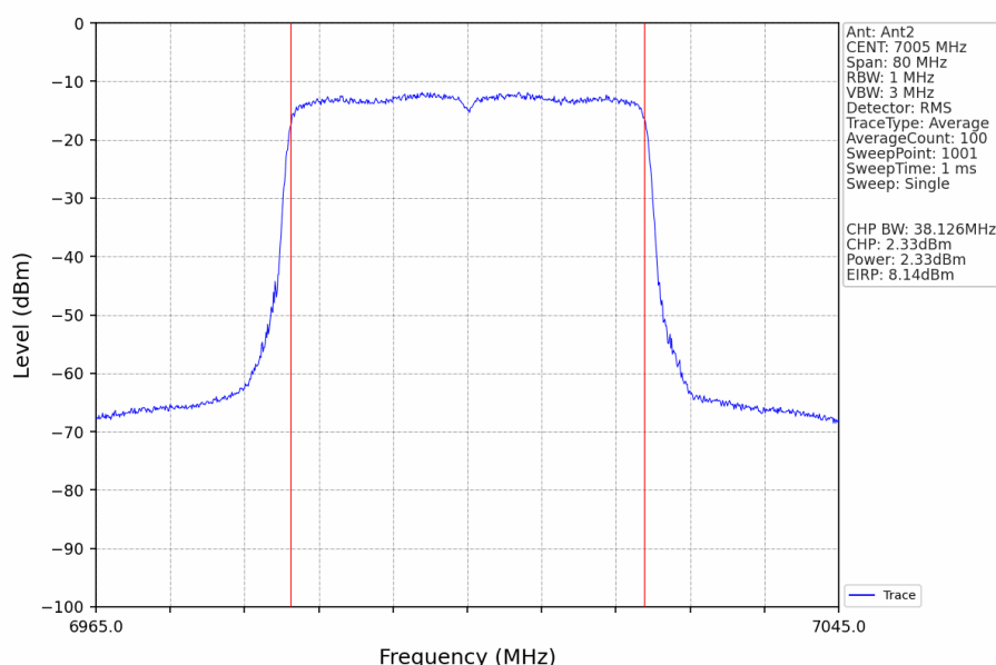
802.11ax(HEW40)_MCH_7005MHz_RU484_Left_Ant2_NTNV
