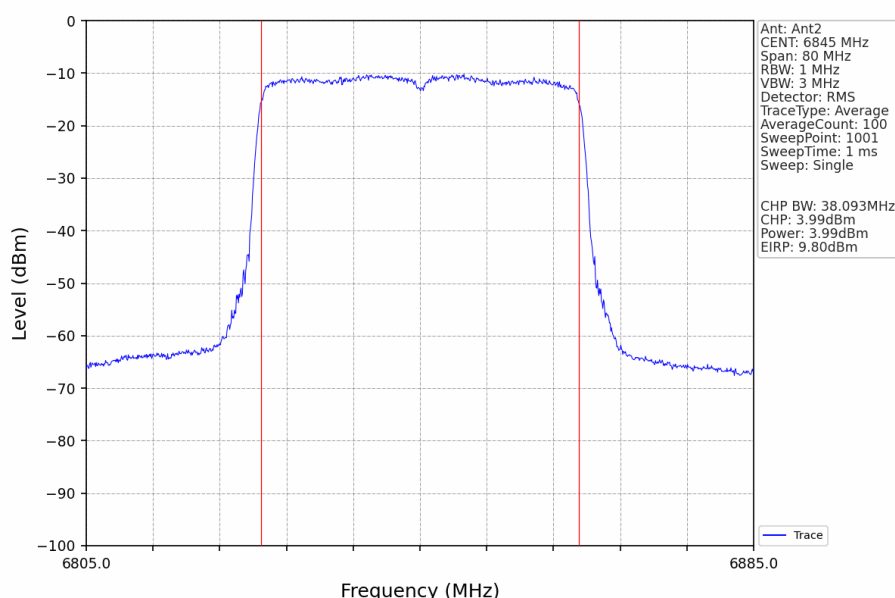
802.11ax(HEW40)_HCH_6845MHz_RU484_Left_Ant2_NTNV
