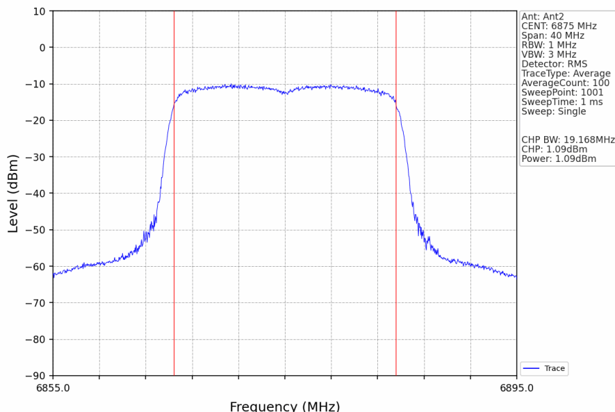
802.11ax(HEW20)_HCH_6875MHz_RU242_Left_Ant2_NTNV
