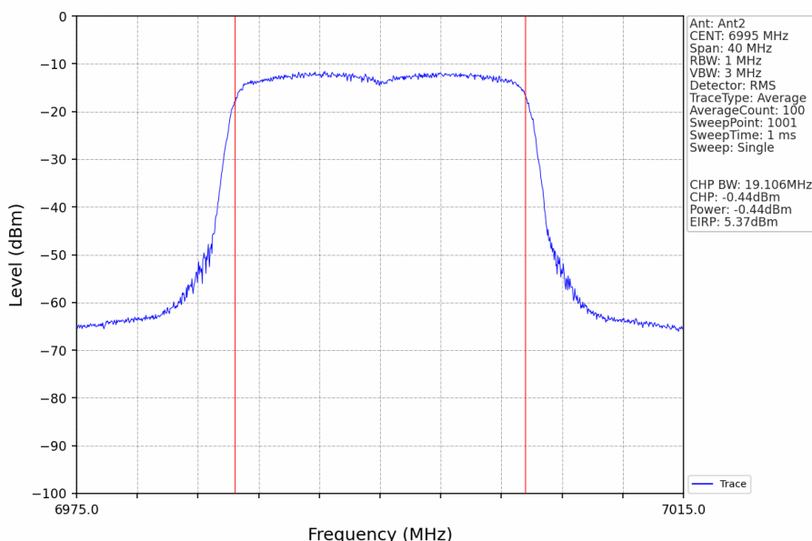
802.11ax(HEW20)_MCH_6995MHz_RU242_Left_Ant2_NTNV
