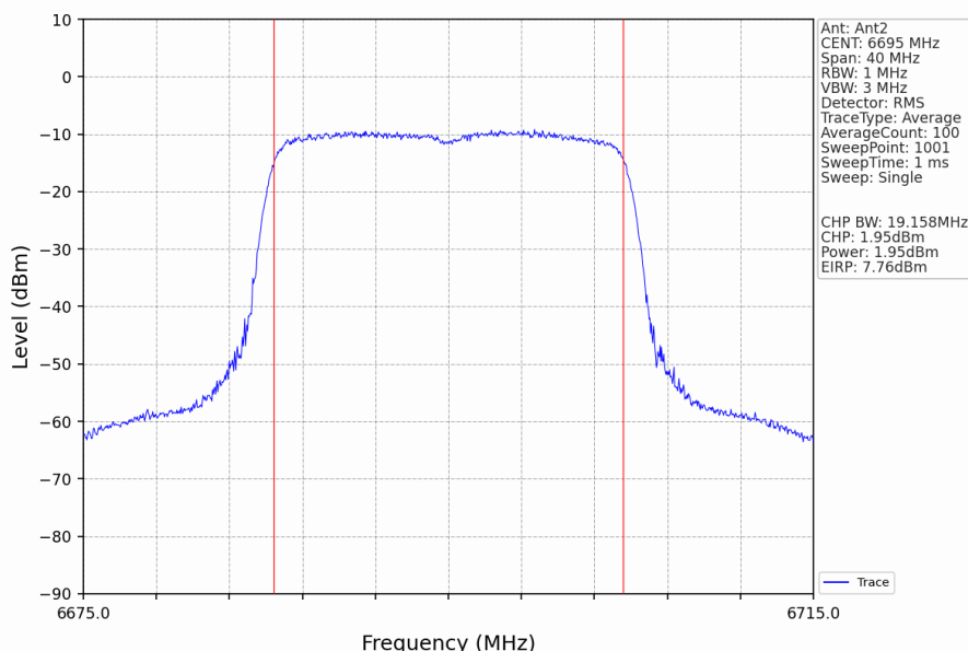
802.11ax(HEW20)_MCH_6695MHz_RU242_Left_Ant2_NTNV
