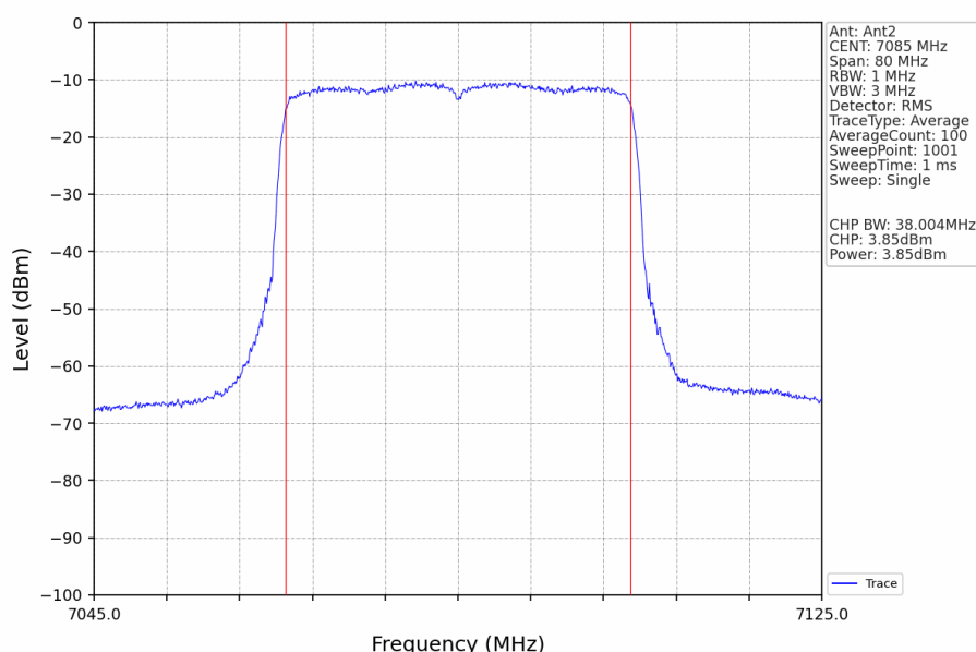
802.11ax(HEW40)_HCH_7085MHz_RU484_Left_Ant2_NTNV
