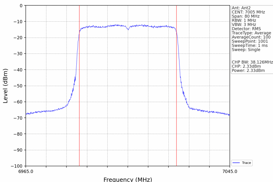
802.11ax(HEW40)_MCH_7005MHz_RU484_Left_Ant2_NTNV
