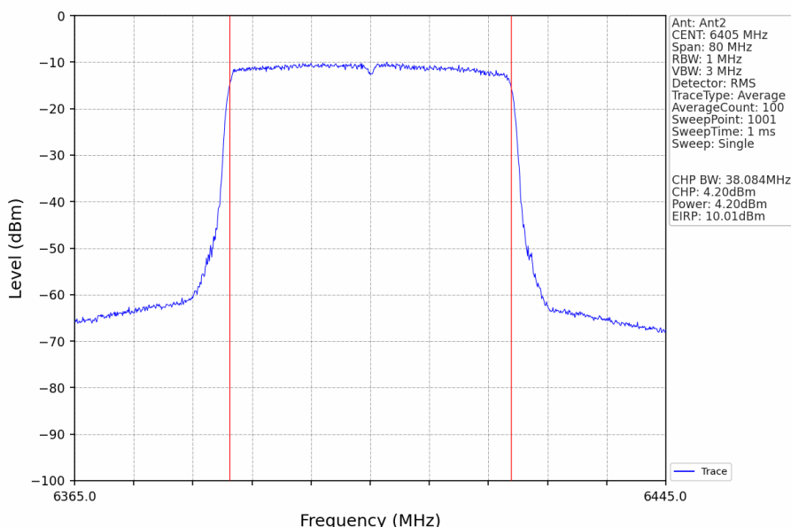
802.11ax(HEW40)_HCH_6405MHz_RU484_Left_Ant2_NTNV
