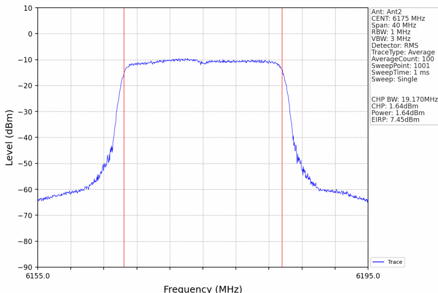
802.11ax(HEW20)_MCH_6175MHz_RU242_Left_Ant2_NTNV
