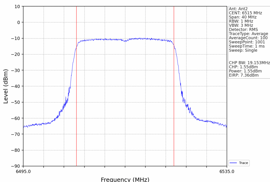
802.11ax(HEW20)_HCH_6515MHz_RU242_Left_Ant2_NTNV
