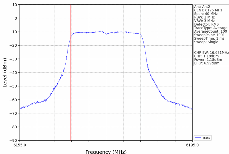
802.11a_MCH_6175MHz_Ant2_NTNV
