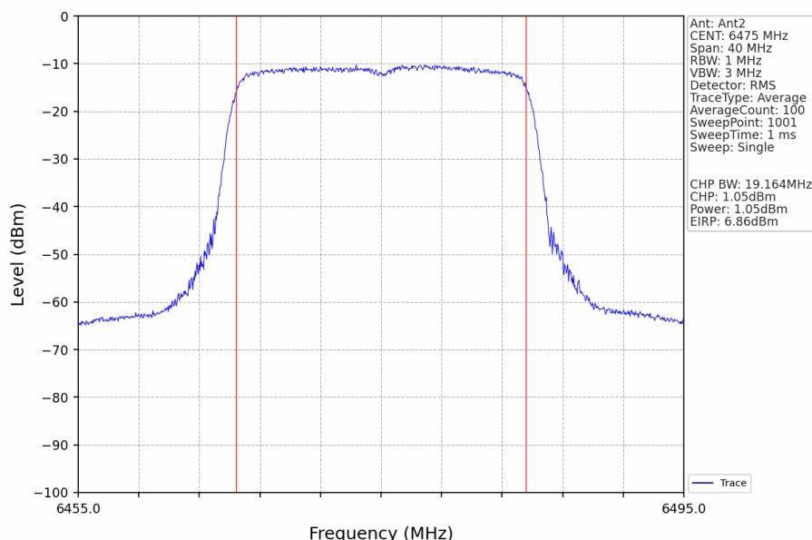
802.11ax(HEW20)_MCH_6475MHz_RU242_Left_Ant2_NTNV
