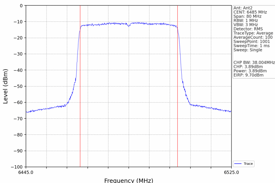
802.11ax(HEW40)_MCH_6485MHz_RU484_Left_Ant2_NTNV
