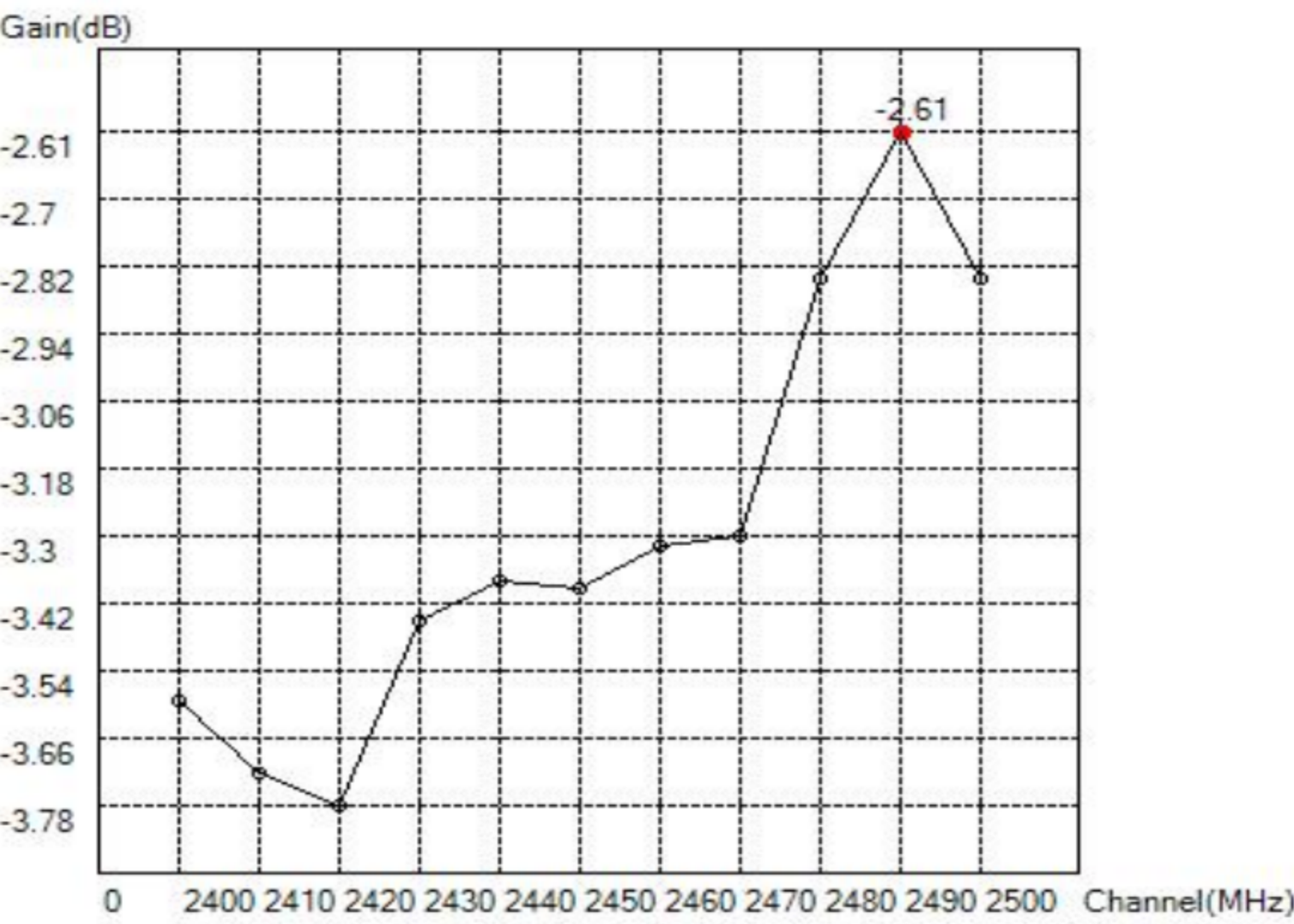
Gain-Plane
