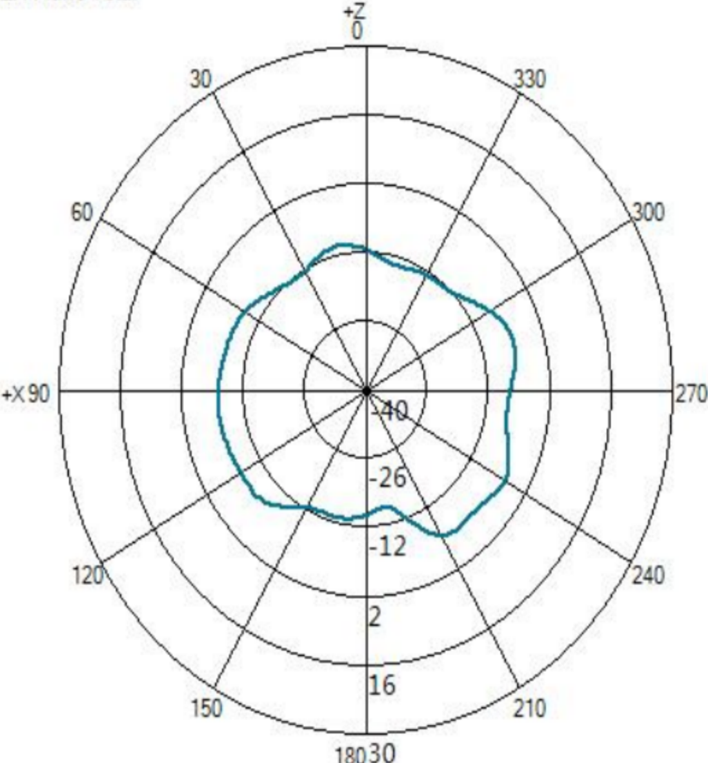
Gain-Plane
