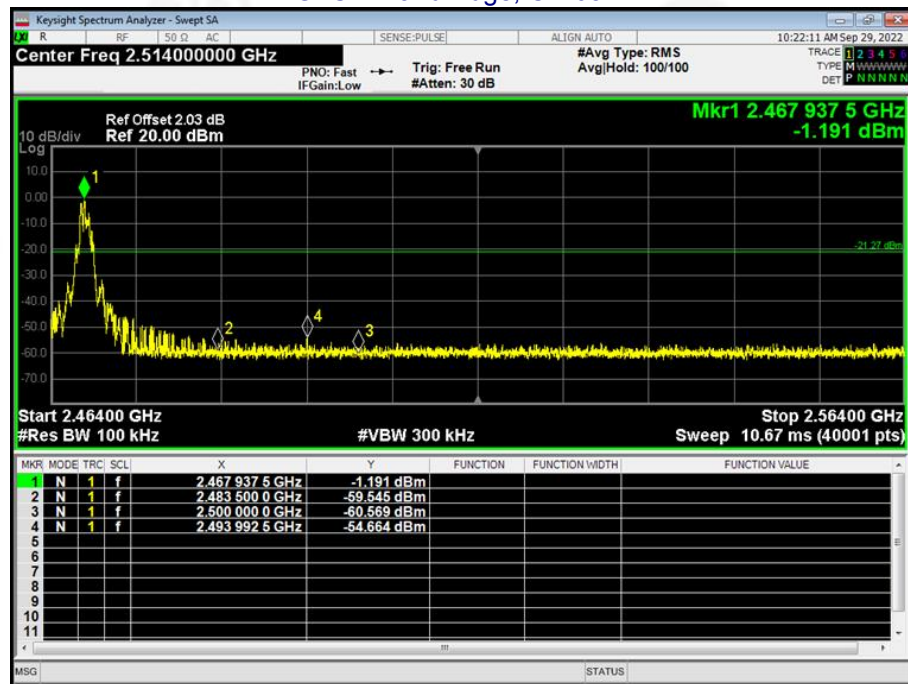
GFSK: Band Edge, CH 03
