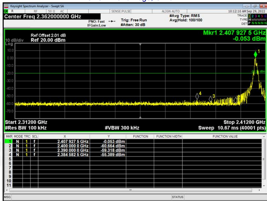
GFSK: Band Edge, CH 01
