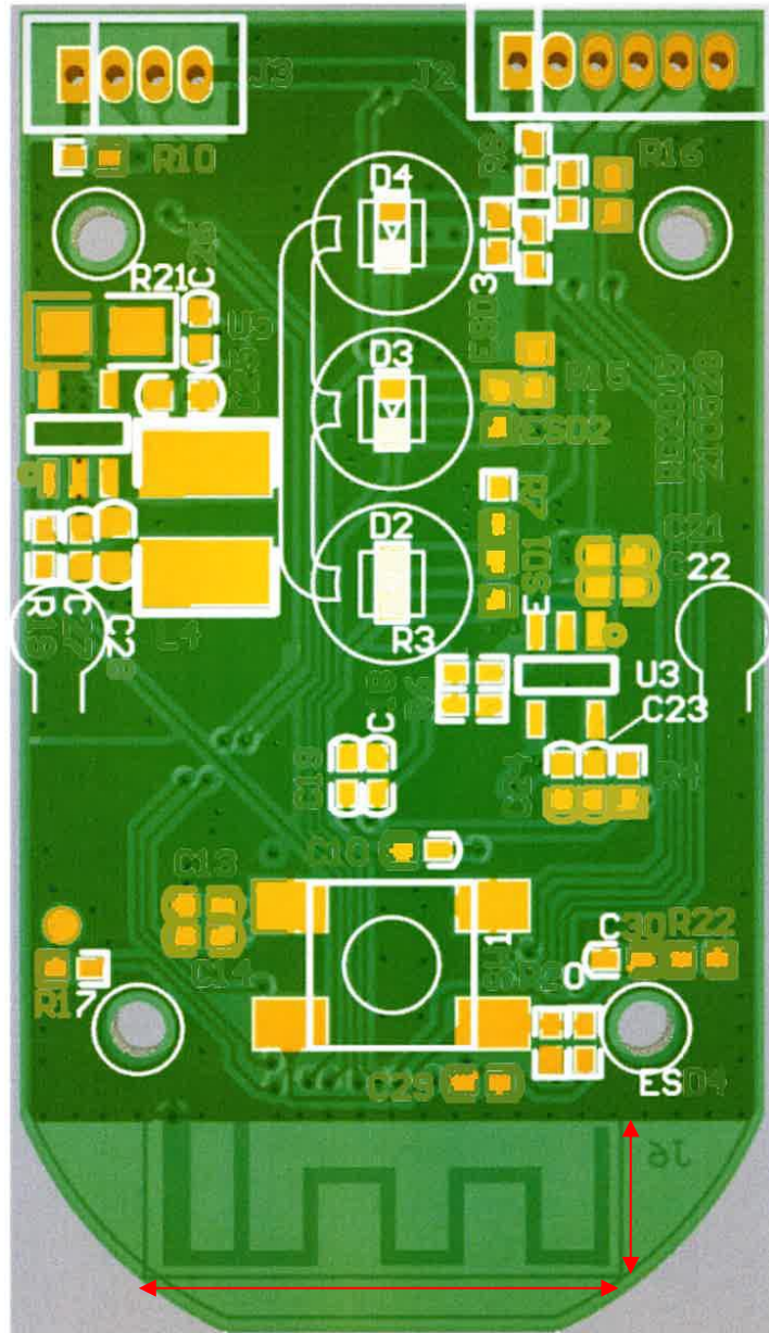
Figure 1 Physical dimension 15*5 (mm)
