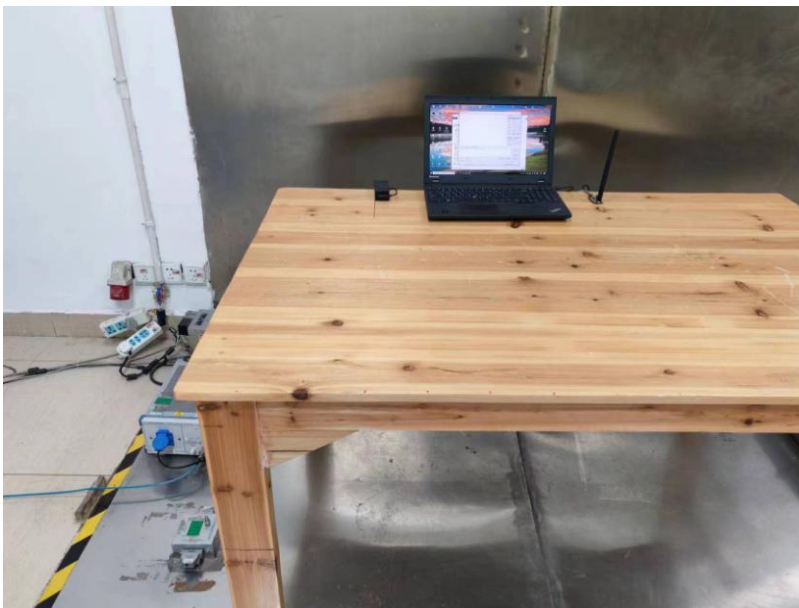
Conducted Emission Setup Front View
