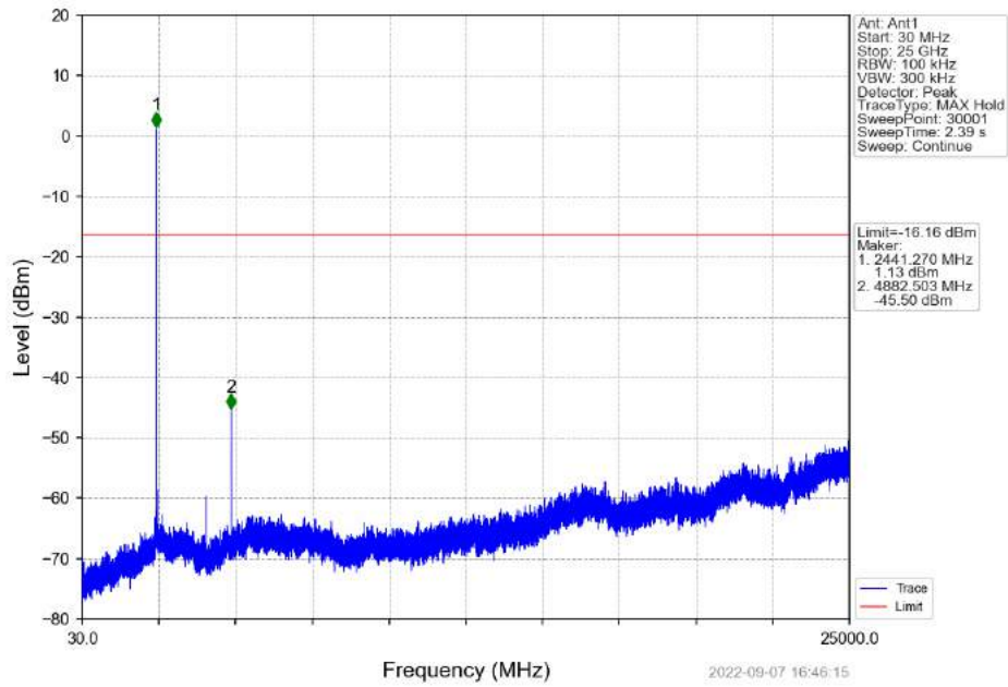
Pi/4DQPSK_2DH5_MCH_2441MHz_Ant1_NTNV
