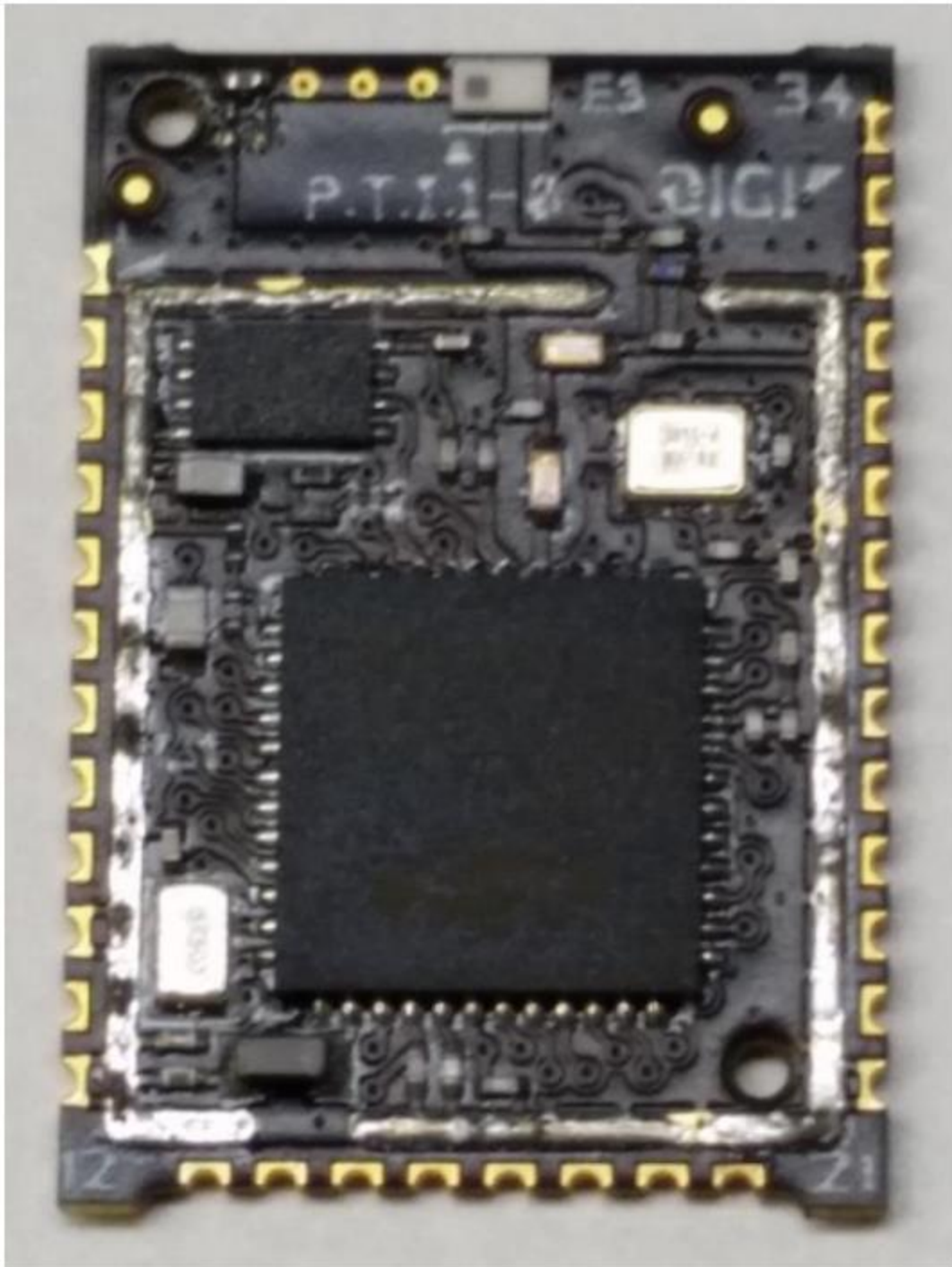
Chip Antenna Interior
