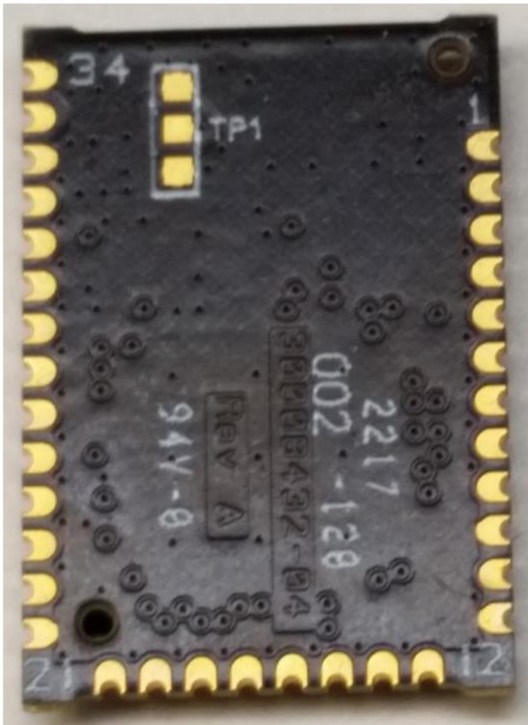
RF Pad Backside
