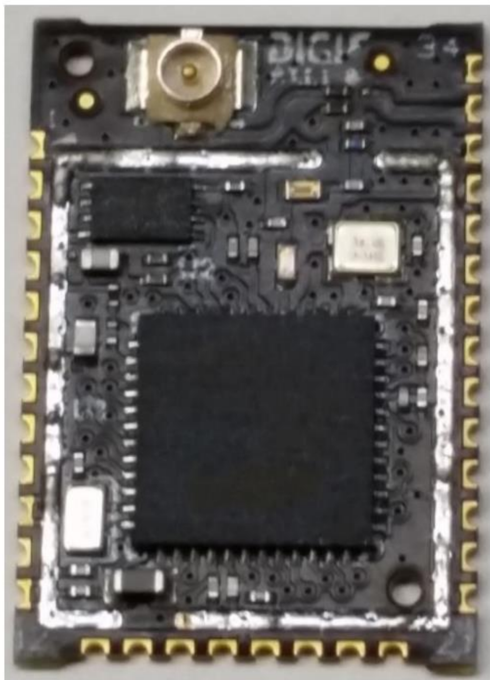
U.FL Interior
