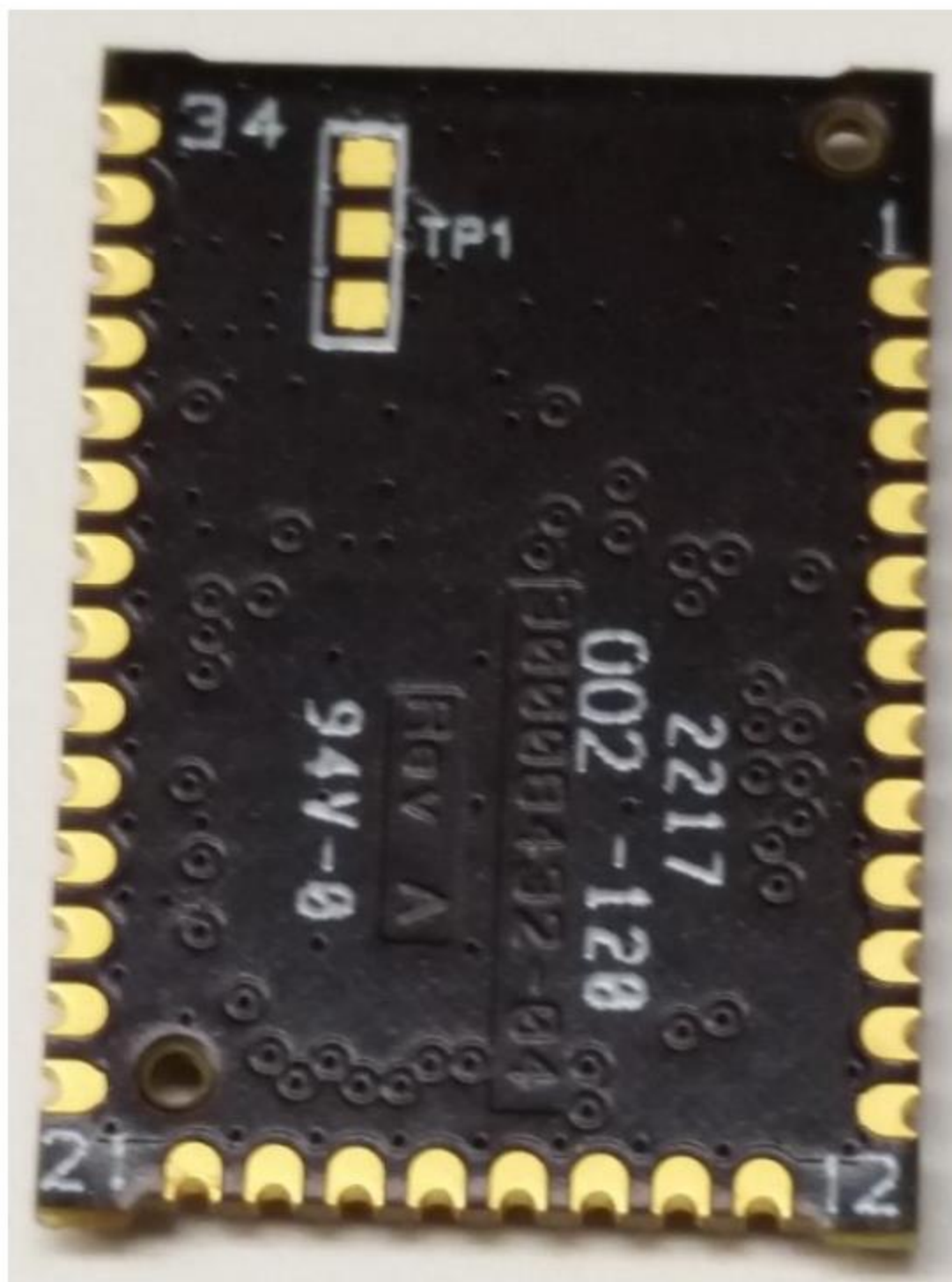
U.FL Backside
