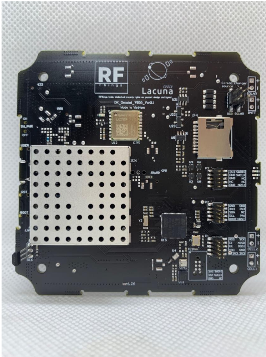
Main PCB (with RF shield)
