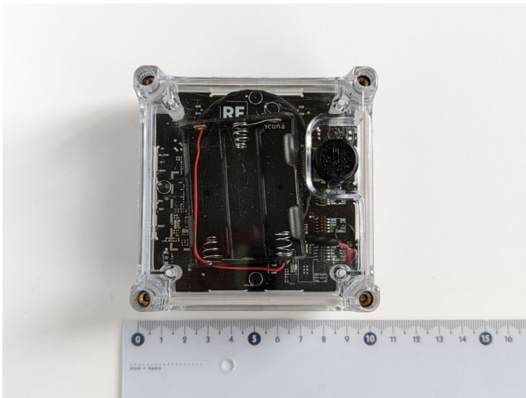
Main PCB (excluding RF shield)
