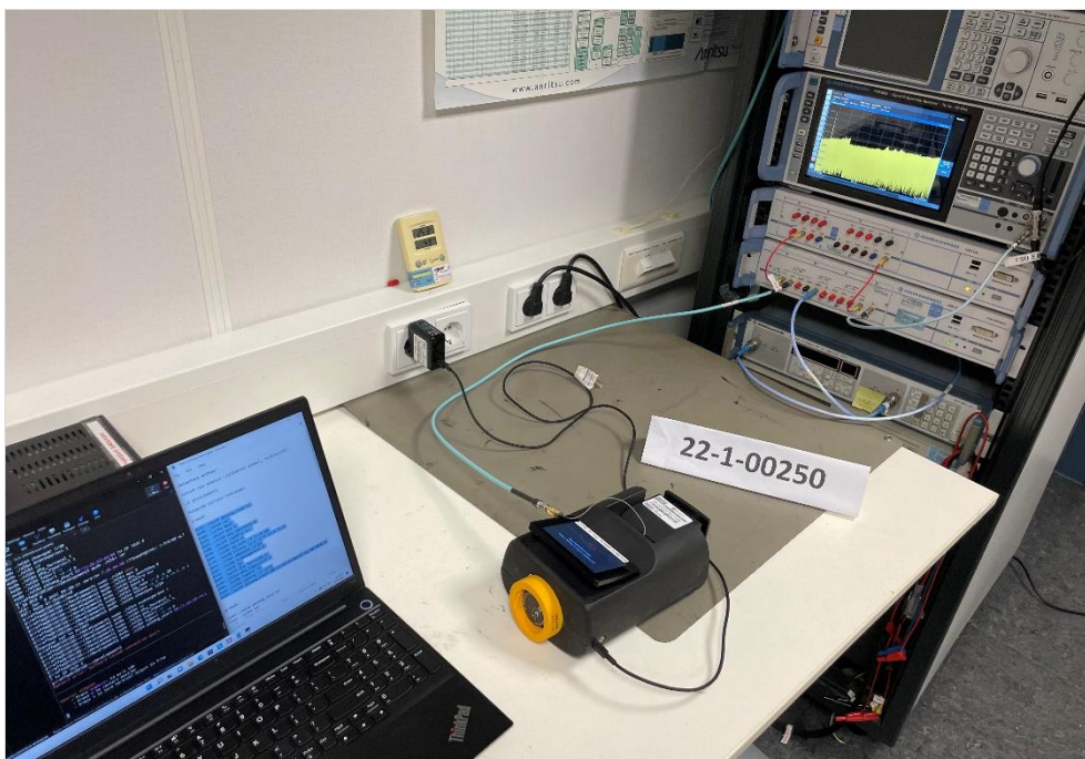
Photograph 2: EUT setup conducted measurement, overview
