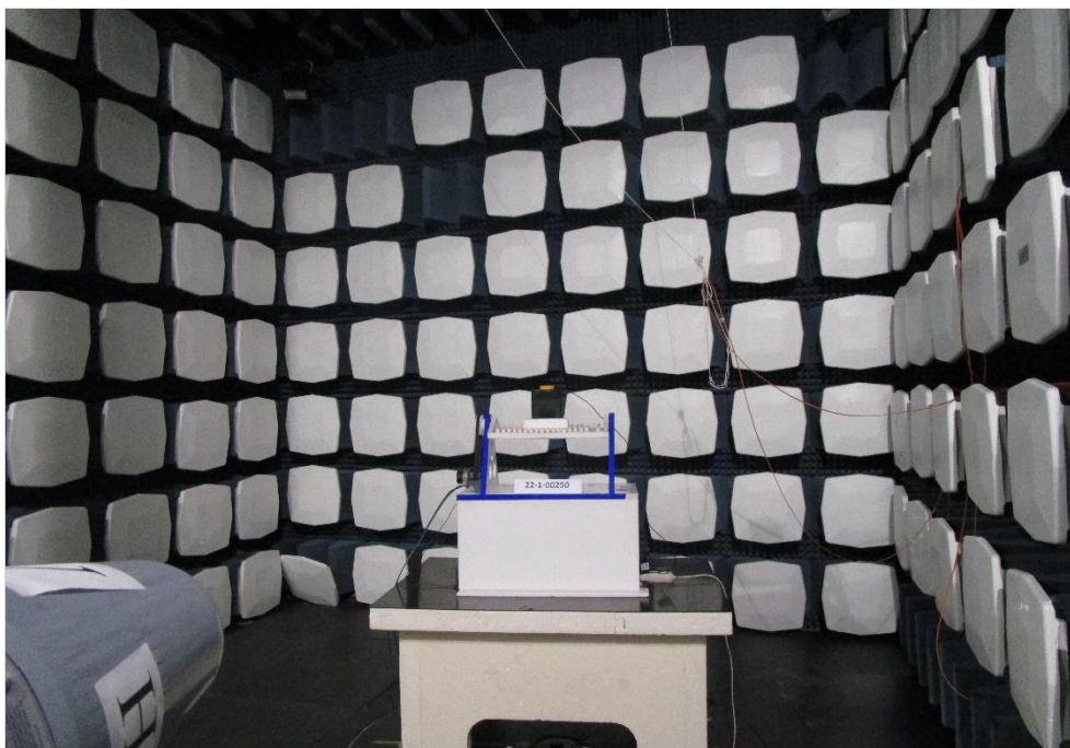
Photograph 10: EUT test setup in the fully anechoic chamber, overview_standing
