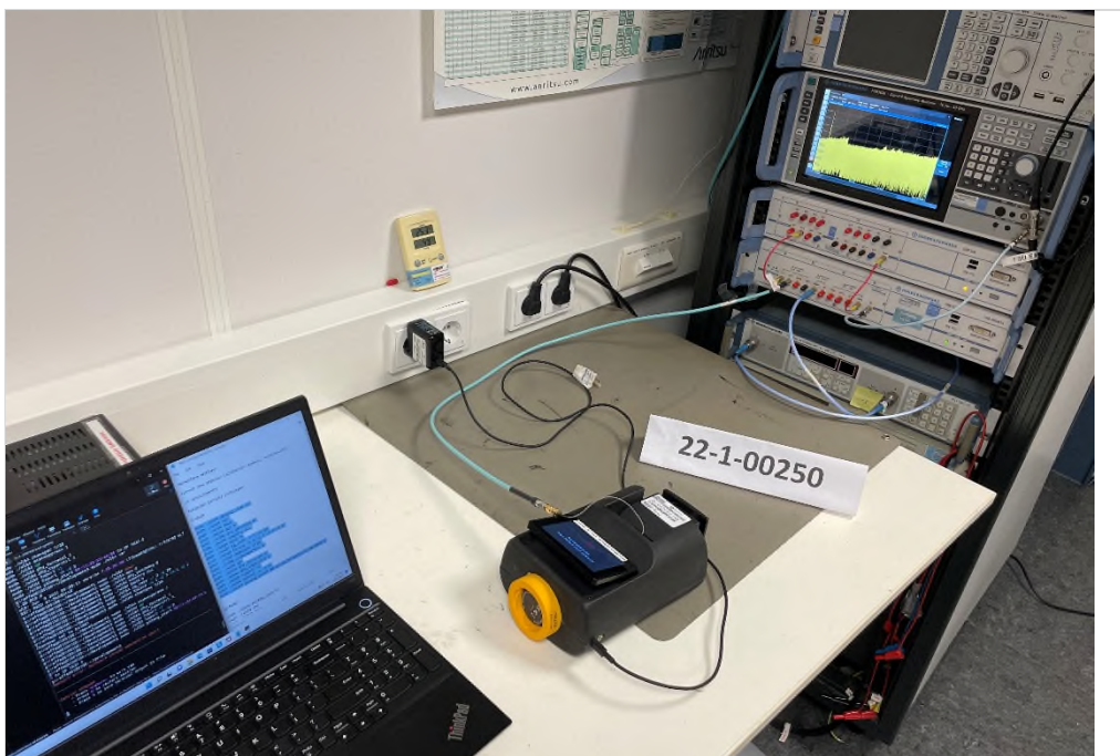
Photograph 2: EUT setup conducted measurement, overview
