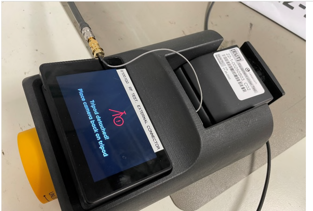
Photograph 1: EUT setup conducted measurement, close up view
