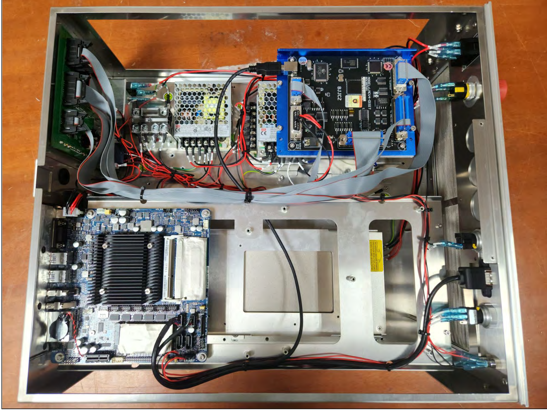
Inside of EUT(CONTROLLER)
