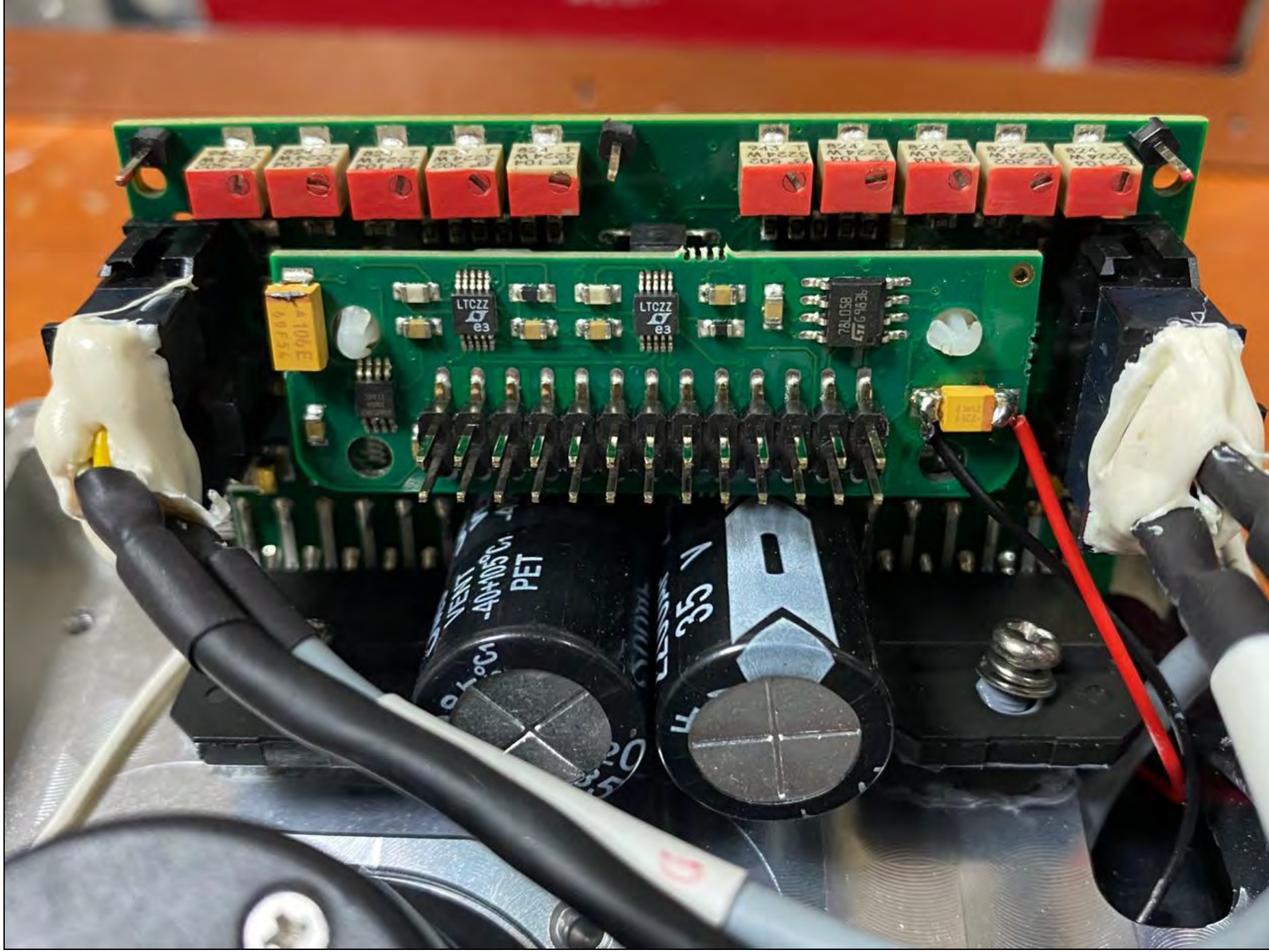
Front View of Laser Head Motor Contrroller Board
