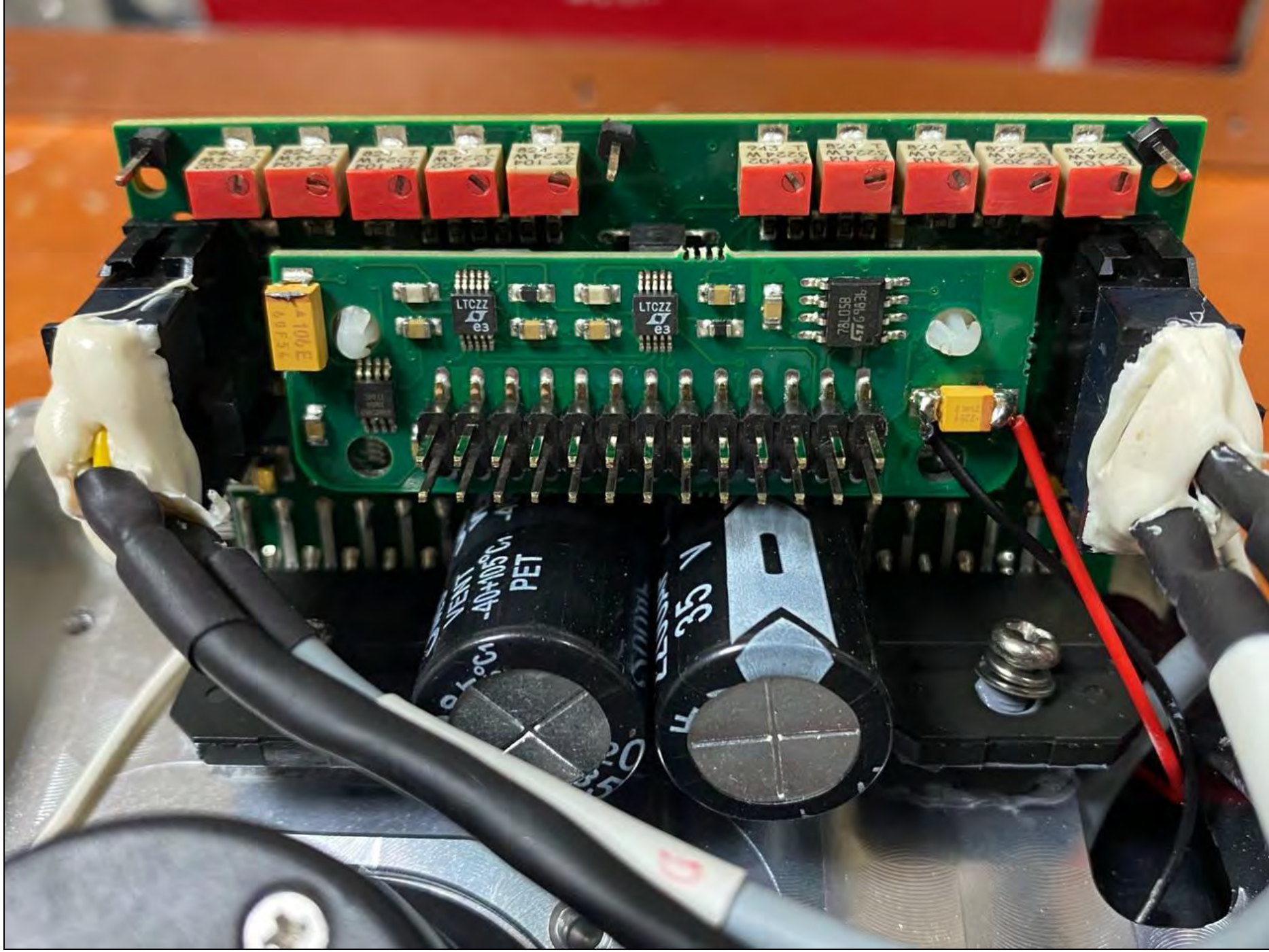
Front View of Laser Head Motor Controller Board
