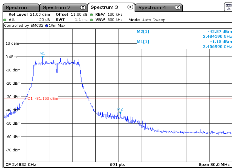
Channel 11: 2.462 GHz
