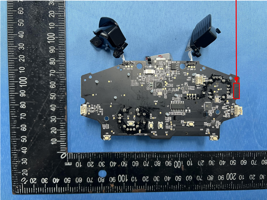
PCB Antenna
