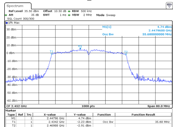
802.11n40_2452MHz
