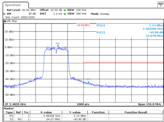
802.11ax20_2462MHz_RU_Full
