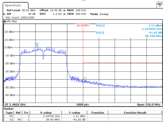
802.11n40_2452MHz
