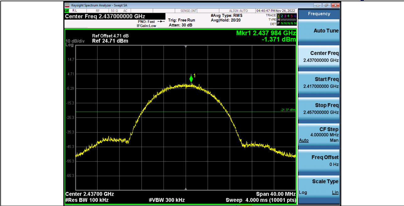
2_Spurious_Emission_2_4GWiFi_NVNT_ANT1_802_11b_2437
