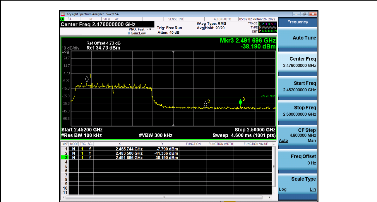
2_Bandedge_2_4GWiFi_NVNT_ANT1_802_11n(HT20)_2462
