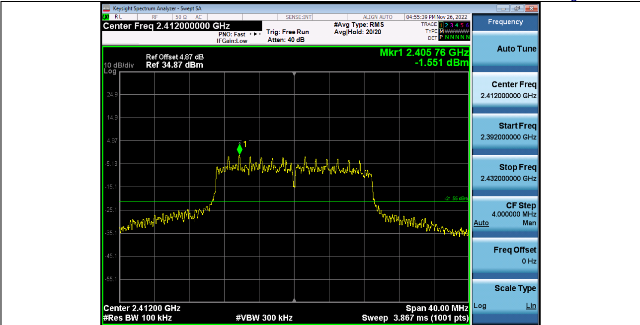
2_Bandedge_2_4GWiFi_NVNT_ANT1_802_11n(HT20)_2412
