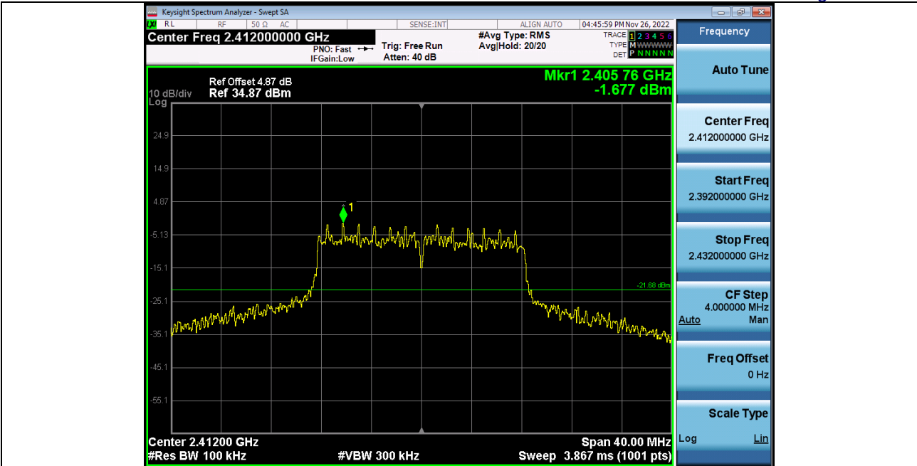
2_Spurious_Emission_2_4GWiFi_NVNT_ANT1_802_11g_2412
