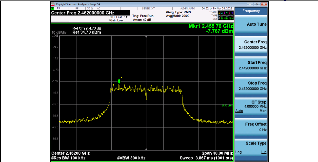
2_Bandedge_2_4GWiFi_NVNT_ANT1_802_11g_2462
