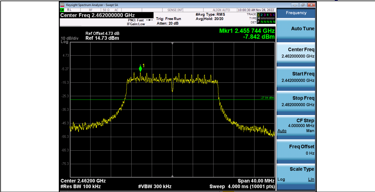
2 Spurious Emission 2 4GWiFi_NVNT_ANT1_802_11n(HT20)_2462
