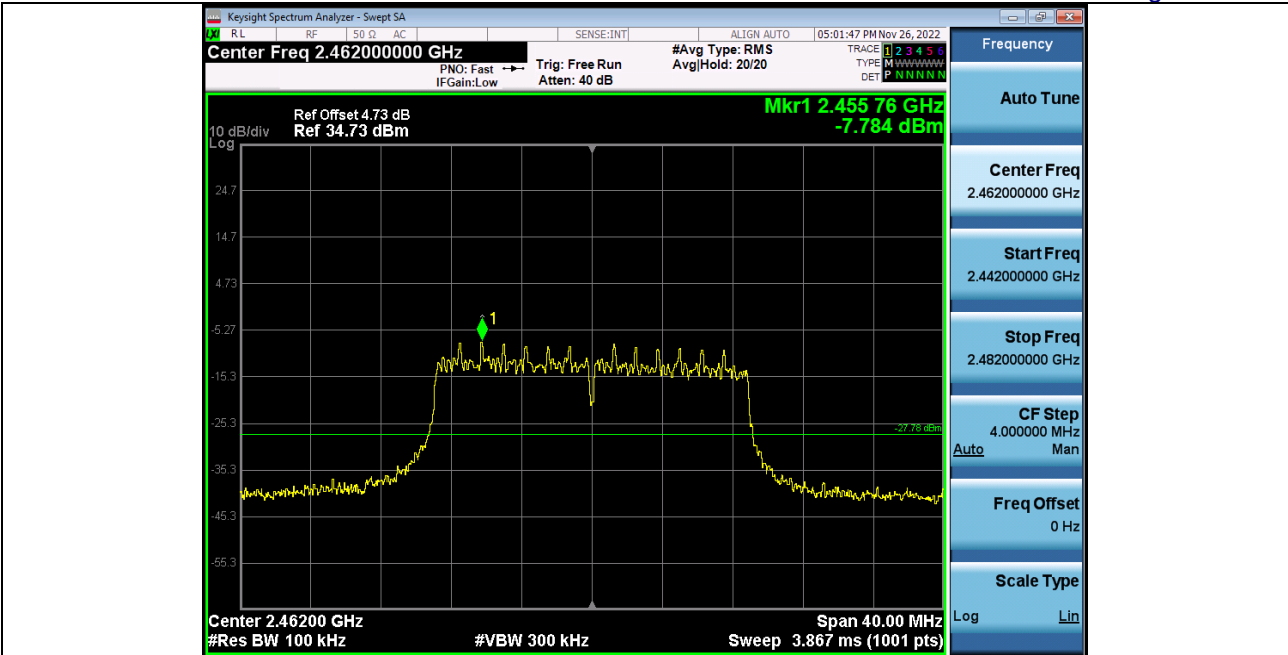
2_Bandedge_2_4GWiFi_NVNT_ANT1_802_11n(HT20)_2462
