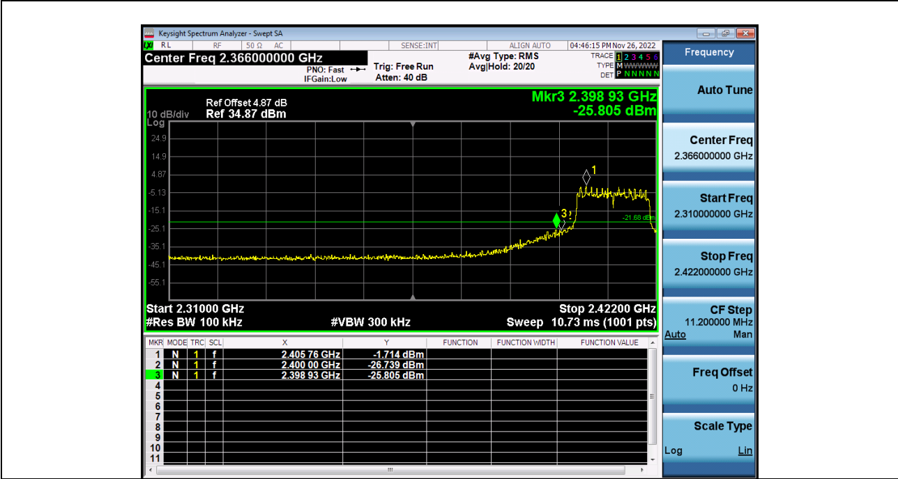
2_Bandedge_2_4GWiFi_NVNT_ANT1_802_11g_2412
