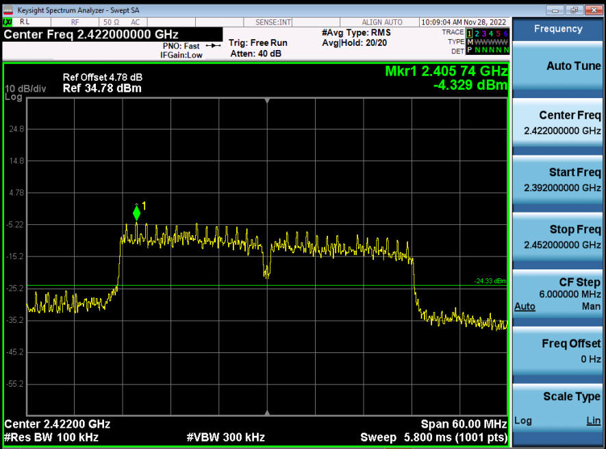
2_Spurious_Emission_2_4GWiFi_NVNT_ANT1_802_11n(HT40)_2422
