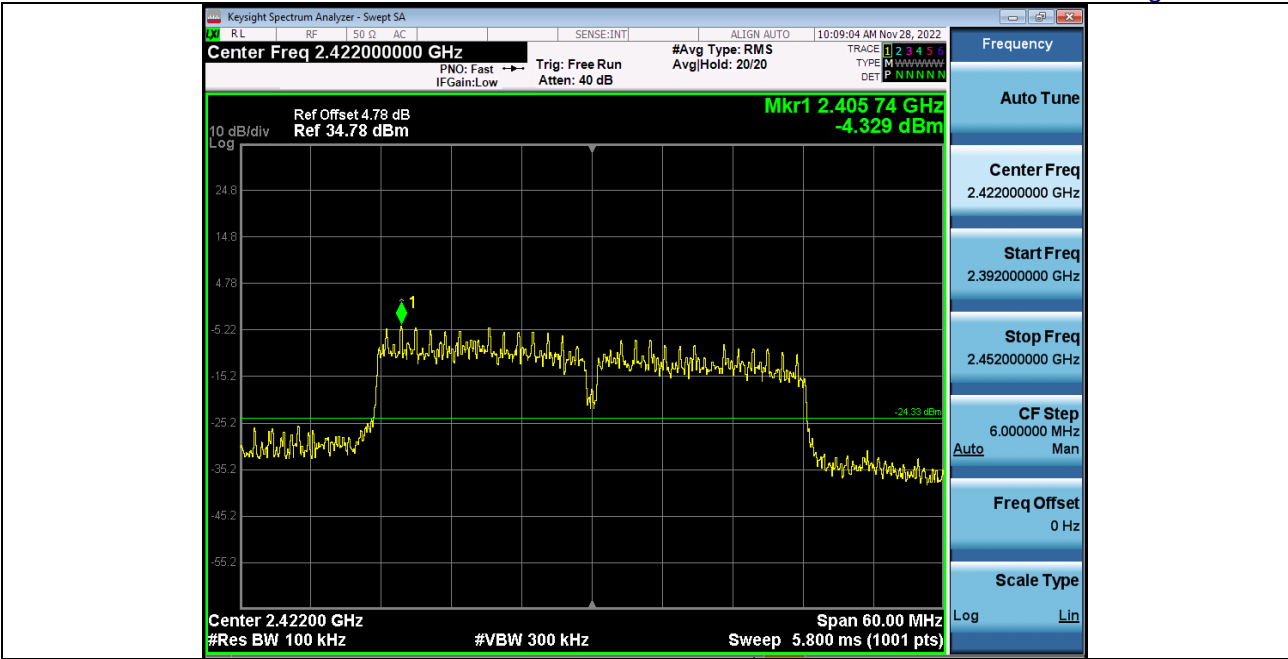
2_Bandedge_2_4GWiFi_NVNT_ANT1_802_11n(HT40)_2422
