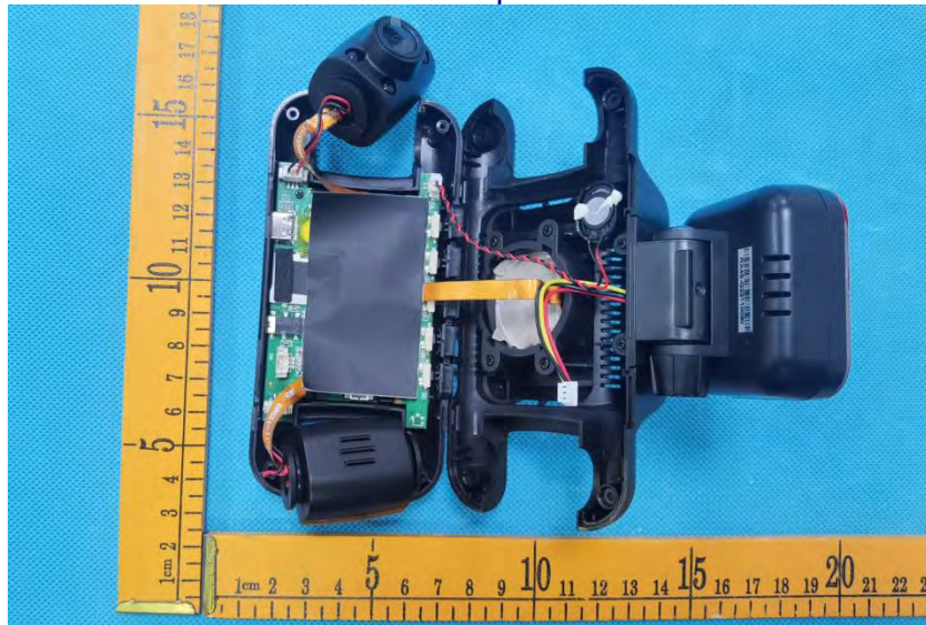
Internal photos
