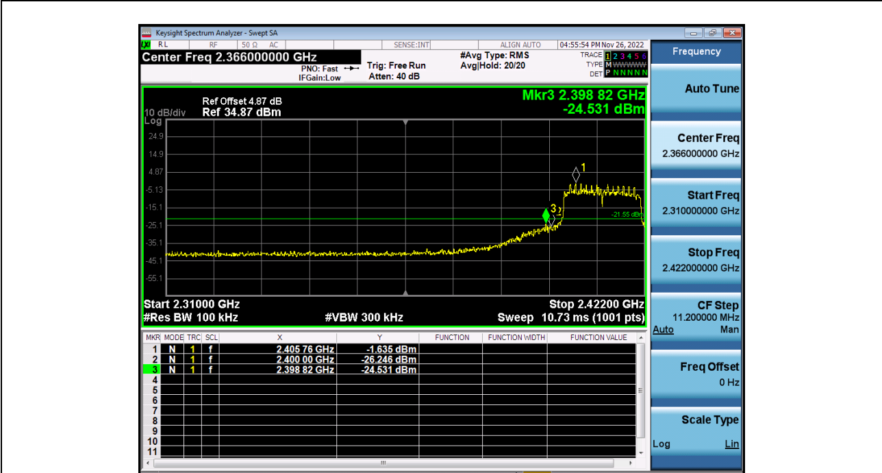
2_Bandedge_2_4GWiFi_NVNT_ANT1_802_11n(HT20)_2412
