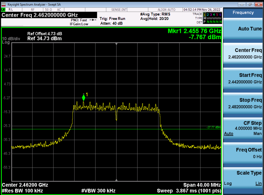
2_Spurious_Emission_2_4GWiFi_NVNT_ANT1_802_11g_2462
