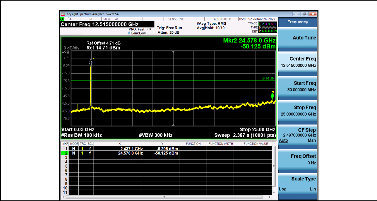
2_Spurious Emission_2_4GWiFi_NVNT_ANT1_802_11n(HT20)_2437
