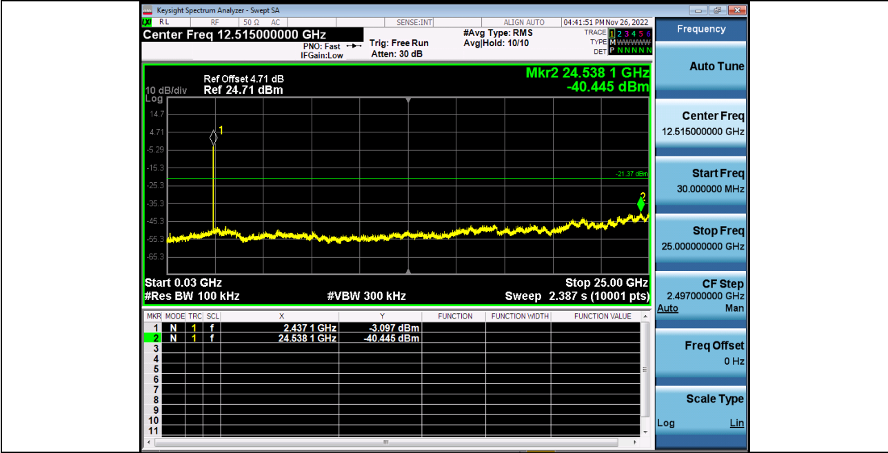
2_Spurious_Emission_2_4GWiFi_NVNT_ANT1_802_11b_2437
