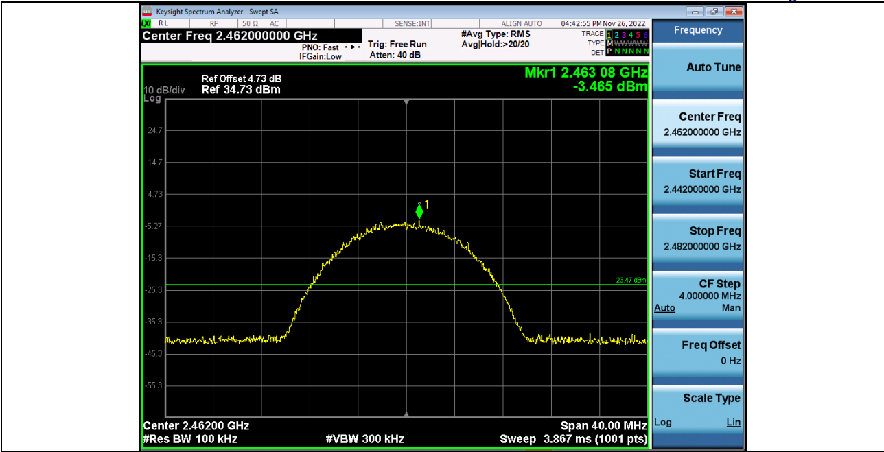
2_Bandedge_2_4GWiFi_NVNT_ANT1_802_11b_2462
