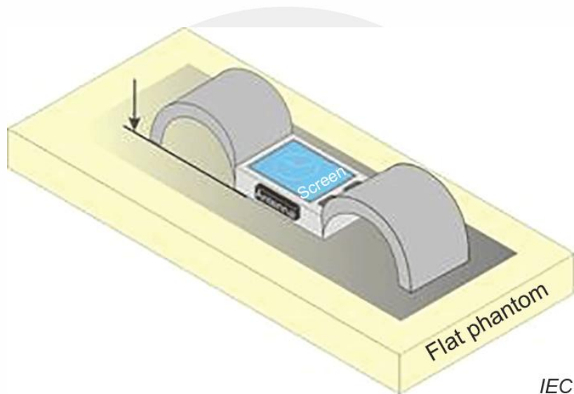
Fig-4.1 Test position for limb-worn devices
