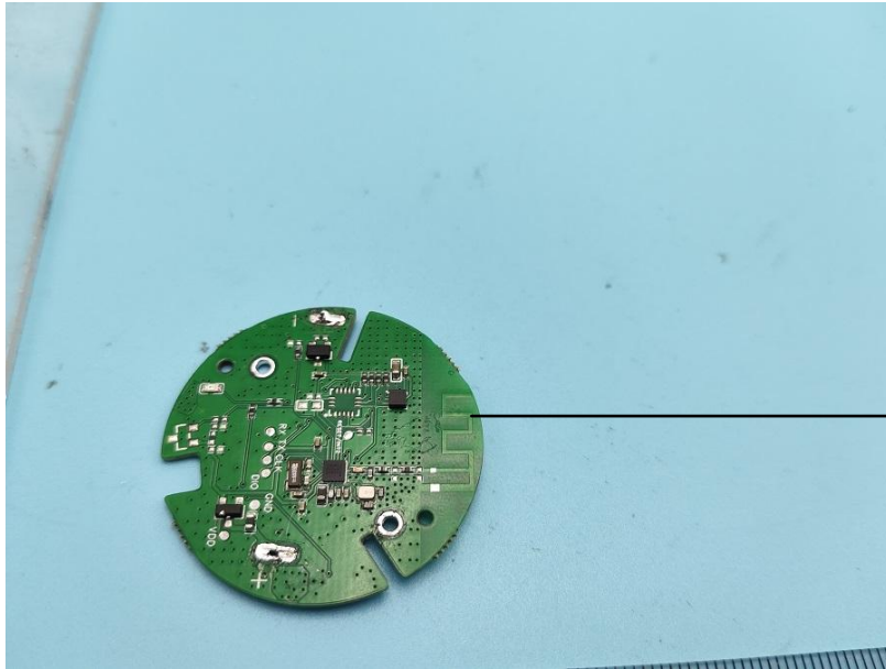
Antenna 2402-2480MHz
