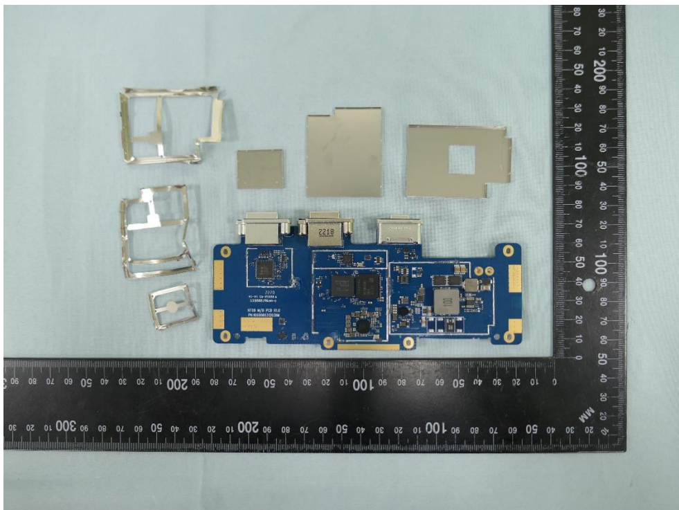
(38) EUT Photo
