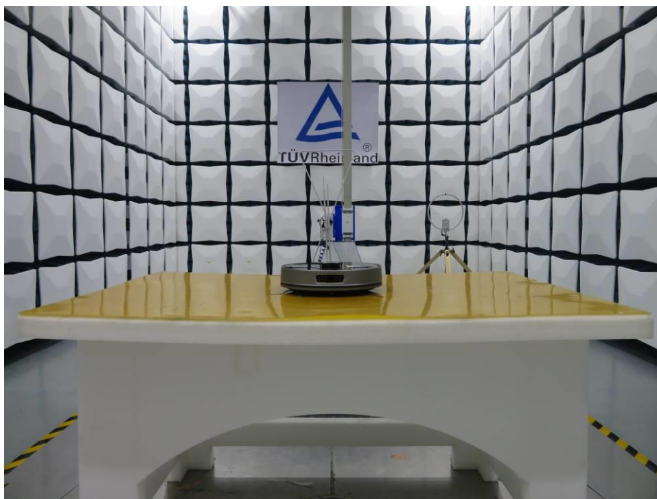
Photograph 1: Set-up photo for Radiated Spurious Emission, up to 1GHz
