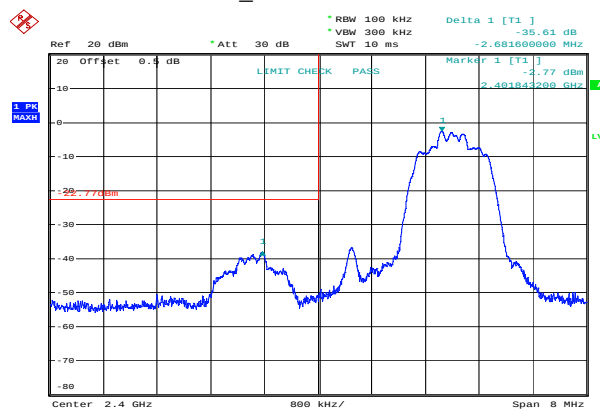
8DPSK_Low 35.61 dB
