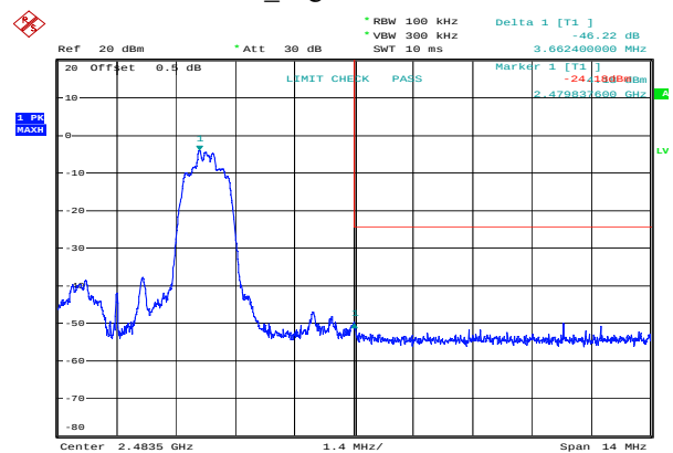
8DPSK_High 46.22 dB
