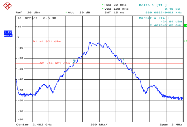
GFSK_Low 0.890 MHz
