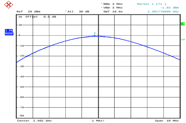
8DPSK_Low -1.03 dBm
