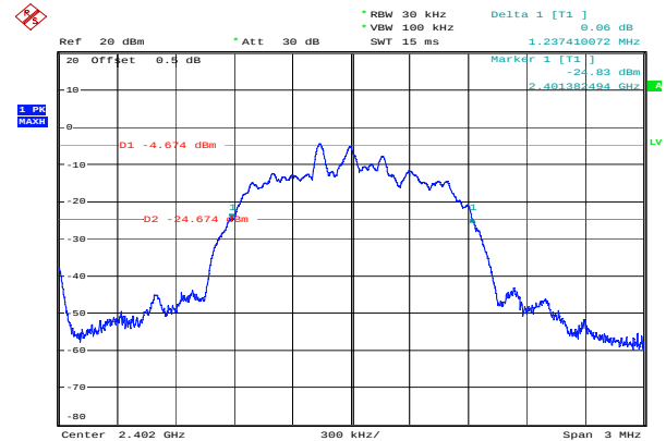
8DPSK_Low 1.237 MHz
