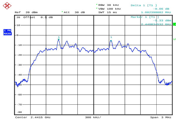
8DPSK_Middle 1.002 MHz
