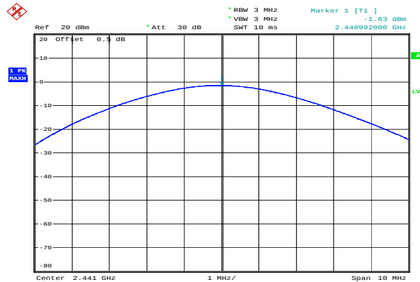
8DPSK_Middle -1.63 dBm
