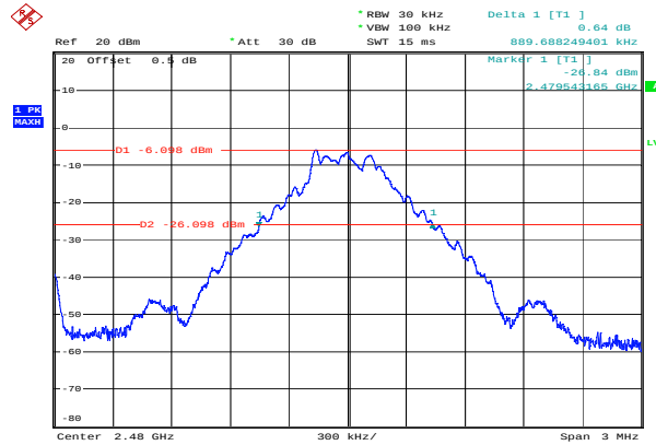
GFSK_High 0.890 MHz
