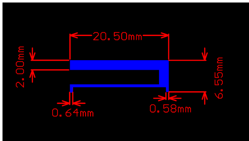
Antenna1 (PCB Antenna)
