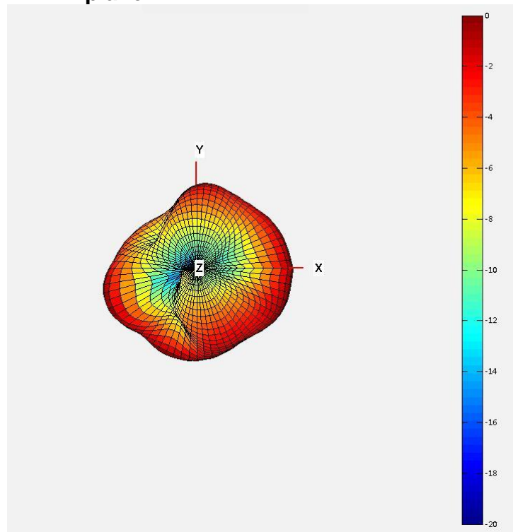
433.92MHz X-Y plane
