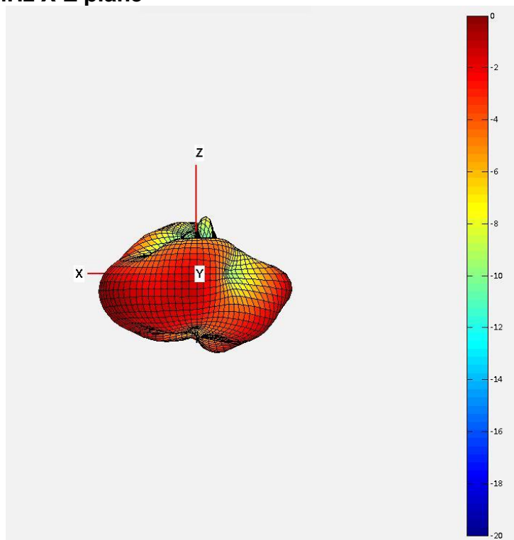
433.92MHz X-Z plane
