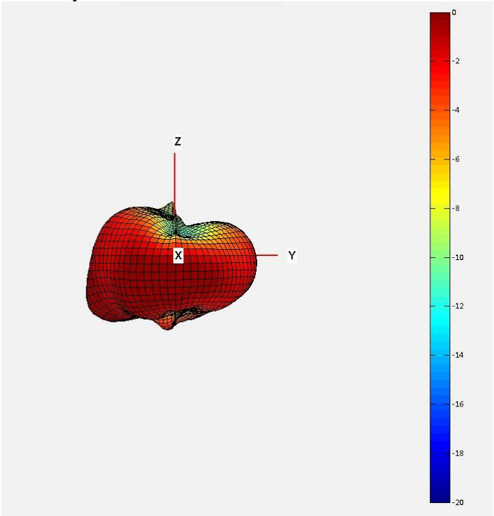
433.92MHz Y-Z plane
