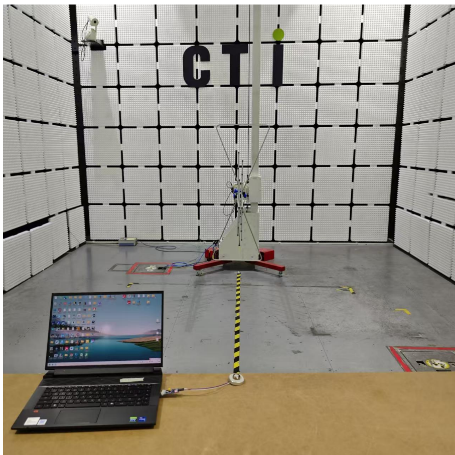
Radiated spurious emission Test Setup-1(Below 1GHz)
