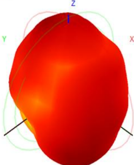
Back View
