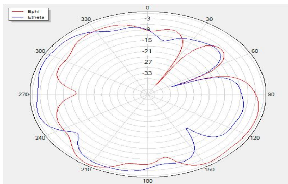
H Theta=90 freq=2430MHz
