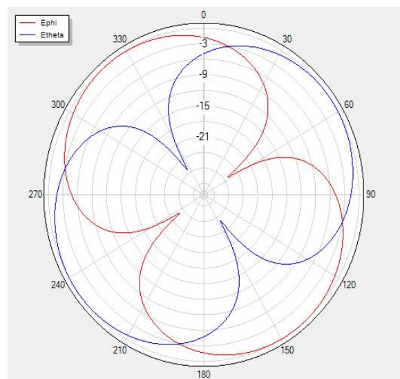
H Theta=0 freq=2480MHz
