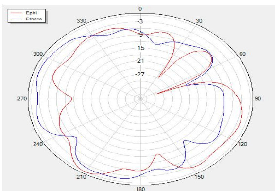
H Theta=90 freq=2450MHz
