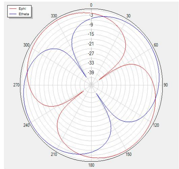
H Theta=0 freq=2460MHz
