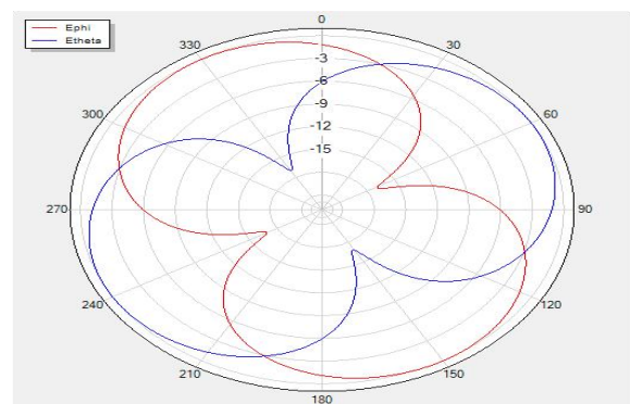
H Theta=0 freq=2410MHz
