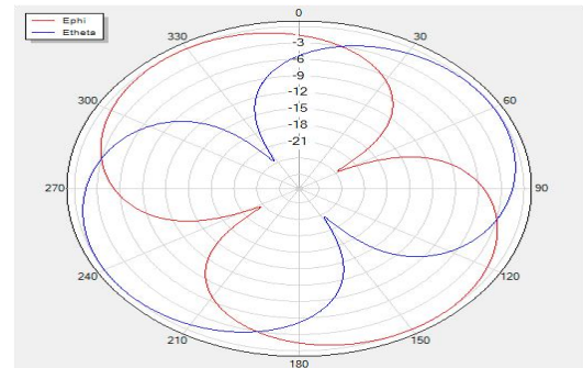
H Theta=0 freq=2440MHz
