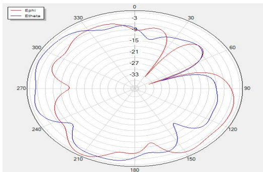
H Theta=90 freq=2440MHz
