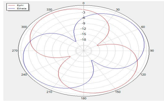
H Theta=0 freq=2420MHz
