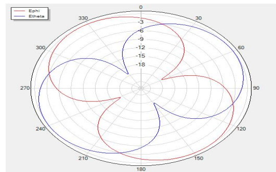
H Theta=0 freq=2430MHz
