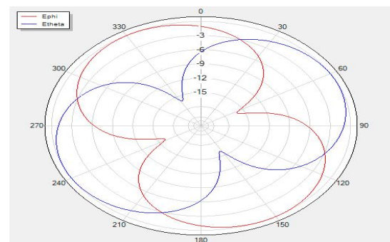
H Theta=0 freq=2400MHz
