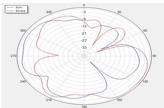
H Theta=90 freq=2410MHz
