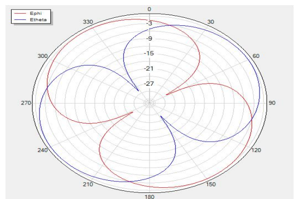
H Theta=0 freq=2450MHz
