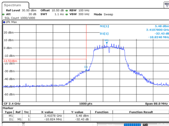
g_2412MHz_Chain 0 32.43dB
