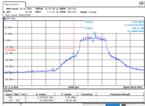
g_2412MHz_Chain 1 30.41dB
