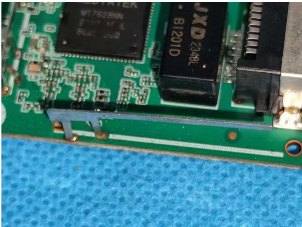
Chain 0 Antenna
