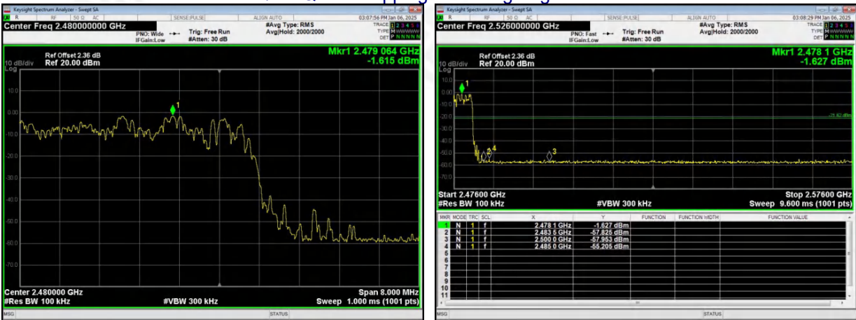
\pi/4 -DQPSK Hopping Band edge-right side
